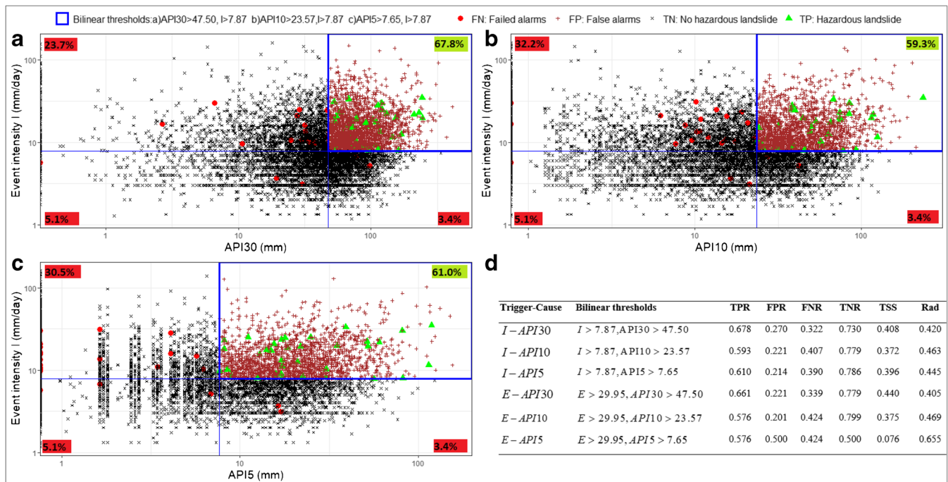
Fig. 6 Bilinear relation between landslide trigger represented by event intensity I and cause represented by antecedent precipitation indices of different timescales. a Thirty days prior to the triggering event intensity. b Ten days prior to the triggering event intensity. c Five days prior to the triggering event intensity. d Implication for warning based on the rate of true warnings (TPR) represented by green triangles on a , b and c ; rate of false alarms (FPR) represented by red cross on a , b and c ; rate of failed alarms (FNR) represented by red dots on a , b and c ; true negative rate (TNR) or no landslide represented by black cross on a , b and c
