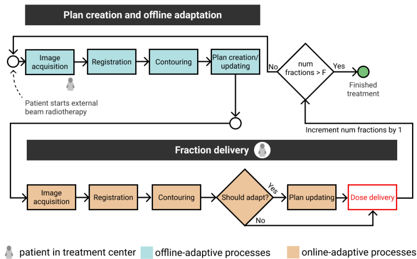
Figure 1. Schematic of external beam radiotherapy (EBRT) dose delivery pipeline. Each box corresponds to one process, and the diamonds to decisions in the workflow. The goal is to deliver the prescribed dose to the patient (red box) in F fractions spread over several days. Adaptive strategies help mitigate dose deviations due to changes in the patient's anatomy during the treatment. Adaptation can be online within a fraction (orange boxes) or offline between fractions (blue boxes).
