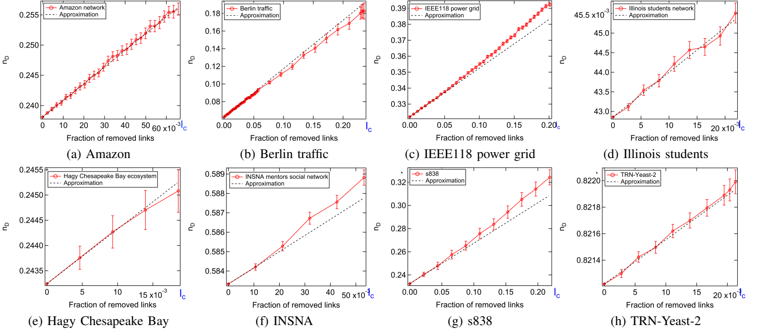
Fig. 2. Performance of the approximation (6) for the normalized minimum number of driver nodes n_D as a function of the fraction of removed links l in real-world networks under random attacks. The results for each fraction l is based on 10000 simulations.
