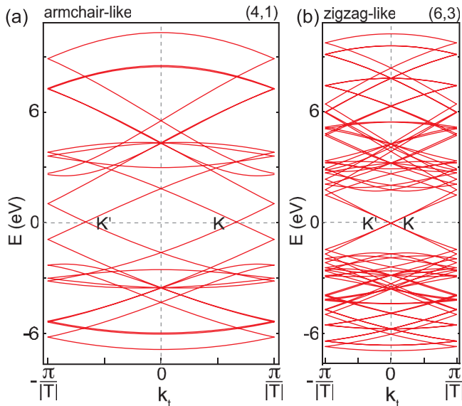
FIG. 6 (color online). Robustness of the valley index in nanotubes. All subbands of the 1D dispersion relation (corresponding to different quantization lines in Fig. 5) are plotted in the first longitudinal Brillouin zone vs longitudinal wave vector k_l . All nominally metallic nanotubes can be classified as armchairlike or zigzaglike. For armchairlike nanotubes, the two Dirac points are separated in k_l ; for zigzaglike nanotubes, they are separated in crystal angular momentum. Since all metallic nanotubes fall into one of these classes, valley is a good quantum number in a slowly varying potential. (a) Armchairlike (4,1) nanotube. (b) Zigzaglike (6,3) nanotube. Each spin-degenerate band is calculated using a graphene tight-binding model taking account of nearest-neighbor overlap integrals but without spin-orbit coupling. Only states near E = 0 participate in transport. Note that the Brillouin zone in (a) has been plotted wider than in (b), to reflect the different longitudinal length |T| of the unit cell in real space.
