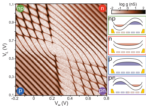
FIG. 25 (color online). Conductance through a narrow-gap nanotube suspended over five gate electrodes that allow independent control over N_L, N_R, \Gamma_L, \Gamma_M , and \Gamma_R . For the gate configuration shown, the nanotube is neutral in the center of the plot ( N_L, N_R ) = (0,0), forms a double quantum dot in the heteropolar regions (top left, bottom right), and forms a single quantum dot in the homopolar regions (top right for electrons, bottom left for holes). Insets visualize the charge distribution along the nanotube for electrons and holes. Adapted from Waissman et al. , 2013, device shown in Fig. 3(f).
