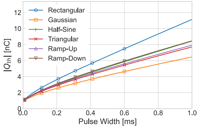
Figure 4. Charge threshold for different pulse shapes and widths in the single-axon fiber model. The pulse widths of the non-rectangular pulses are defined in appendix A.
