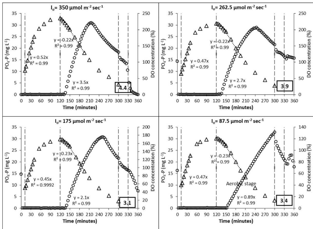
Fig. 8. \text{PO}_4\text{-P} profiles ( \Delta ) combined with online DO profiles ( \circ ) for incident light intensities: 350, 262.5, 175, and 87.5 \mu\text{mol m}^{-2} \text{sec}^{-1} for R1 on days: 83, 86, 89 and 92 of operation, respectively.
