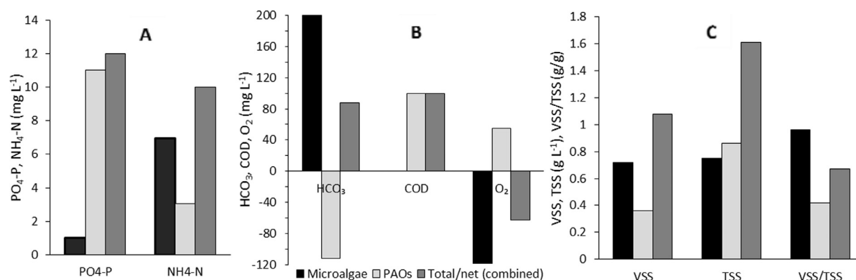
Fig. 1. Model results for: a) influent concentrations of \text{PO}_4\text{-P} and \text{NH}_4\text{-N} ; b) concentrations of \text{HCO}_3^- , COD, and \text{O}_2 (positive values mean consumption/uptake, and negative values mean production/release); and c) the relevant generated biomass (VSS, TSS, VSS/TSS) for microalgae, PAOs and combination.
