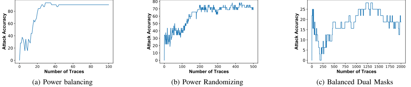
Fig. 6: Countermeasures Analysis using Non-profiled Attacks
