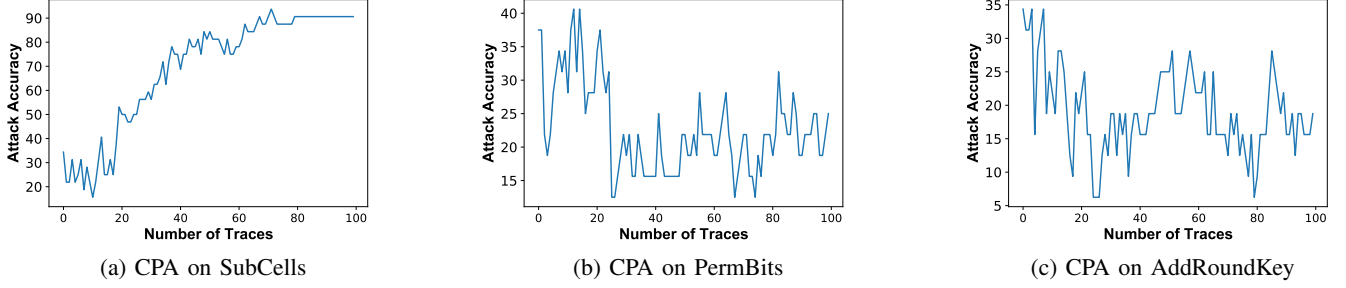
Fig. 4: Accuracy Analysis of Non-profiled Attacks
