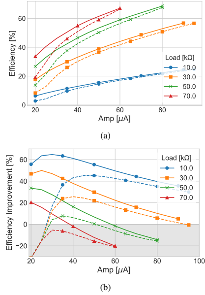
Fig. 9: (a) Simulated schematic (solid) and post-layout (dashed) efficiency of the proposed circuit as a function of output current for 4 load impedances, (b) Efficiency improvement of the proposed circuit with respect to a fixed 5\text{V} -voltage supply
