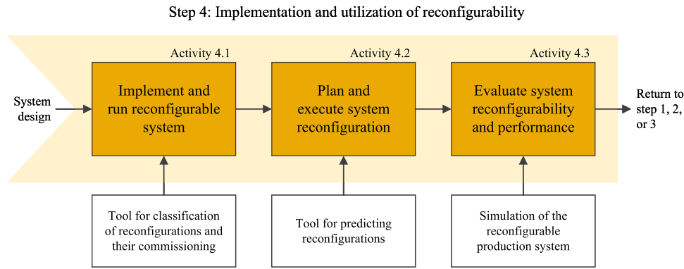
Fig. 8. The fourth step of the proposed development method – “implementation and utilization of reconfigurability” – including its three activities and supporting tools.
