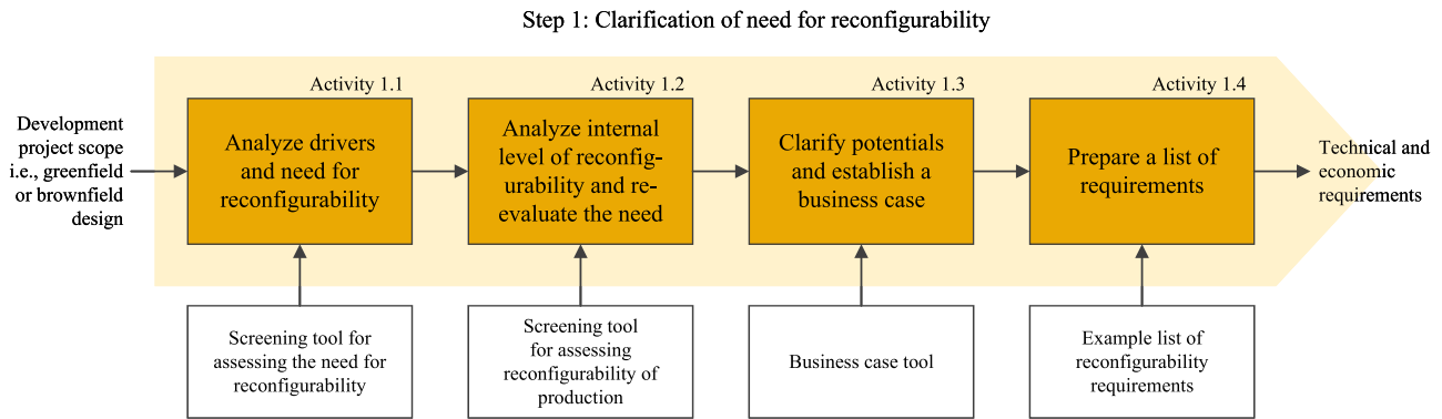
Fig. 5. The first step of the proposed development method – “clarification of need for reconfigurability” – including its four activities and supporting tools and examples.
