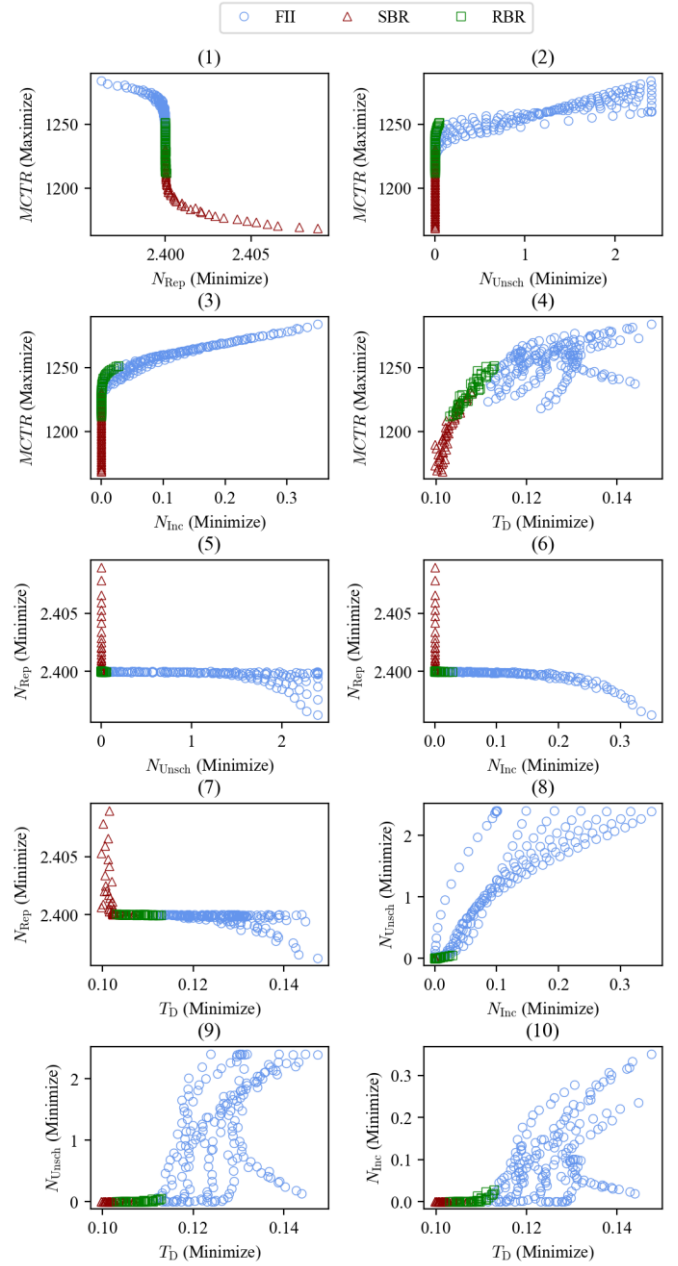
Figure 3. Pairwise objectives of the aircraft maintenance for the FII, SBR and RBR strategies.
