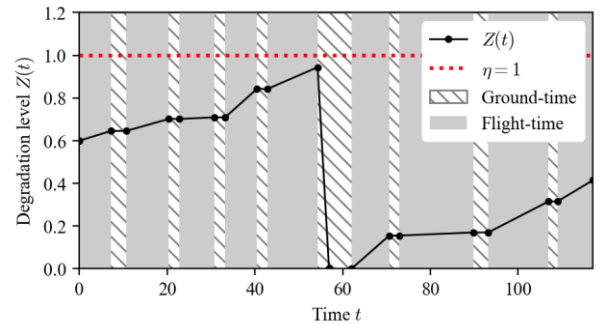
Figure 2. Example of component degradation over time.
