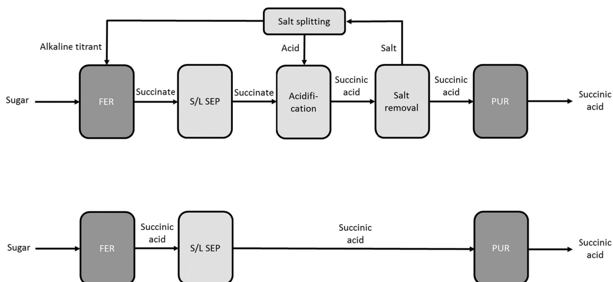
Fig. 3. Succinic acid process configurations. Top: process based on neutral pH fermentation, with a salt splitting step, e.g. via electrochemical or thermal salt treatment. Bottom: process with low pH fermentation (based on Jansen and van Gulik, 2014). FER = fermentation, S/L SEP = solid/liquid separation, PUR = purification.
