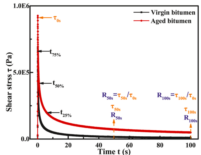
Fig. 3. The representative relaxation curves of virgin and aged bitumen.
