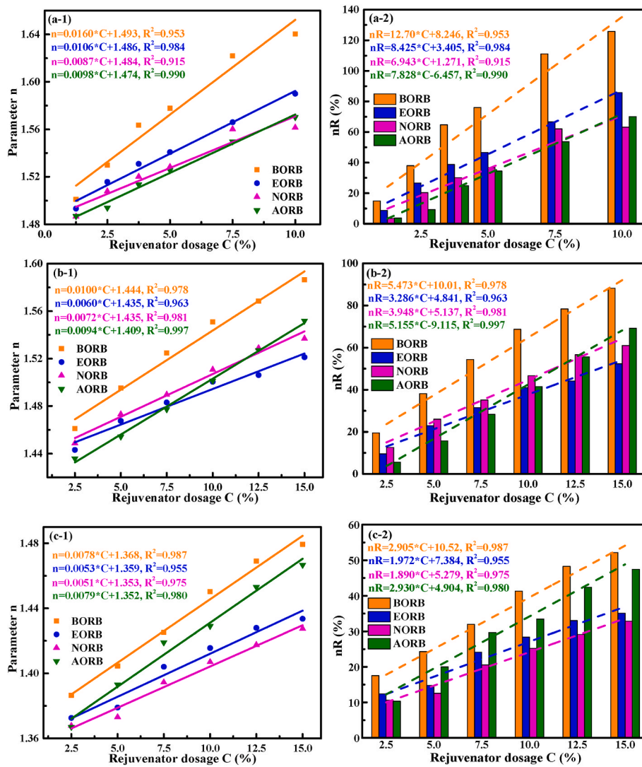
Fig. 15. The parameter n and nR values of various rejuvenated bitumen.
