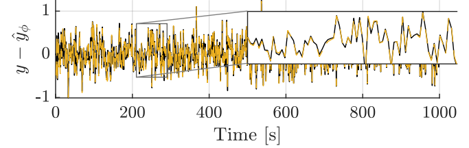
Fig. 3. Prediction residuals y - \hat{y}_\phi (—) and noise realization y - \hat{y} (—) for the validation dataset. The prediction residuals coincide with the noise, i.e., the LPV-IO model (1) with neural network coefficient functions is able to learn all dynamics while simultaneously guaranteeing stability.
