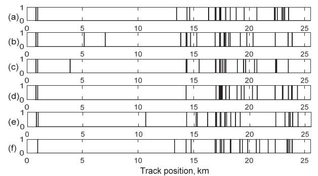
Fig. 10. Optimal Pareto solutions for the rail maintenance decisions. The x-axis depicts the track distance (km) versus the maintenance decision, where 1 represents replacement and 0 represents no replacement. The following algorithms were used: (a) ARMOEA, (b) NSGAI, (c) GrEA, (d) SPEA2, (e) RSEA, and (f) VaEA.
