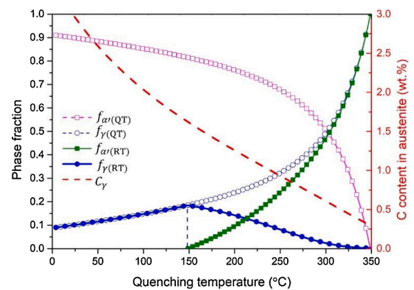
Fig. 16. Phase fraction and carbon content in austenite as a function of quenching temperature predicted by the CCE model for an Fe-0.3C-1.5 Mn-1.5Si steel [12,138]. f_{\gamma}(QT) , f_{\alpha'}(QT) , f_{\gamma}(RT) , f_{\alpha'}(RT) and C_{\gamma} represent the calculated fractions of austenite and martensite at the quench temperature after the first quenching, and fractions austenite and martensite at room temperature after the final quenching, and the calculated carbon content in austenite after partitioning.
