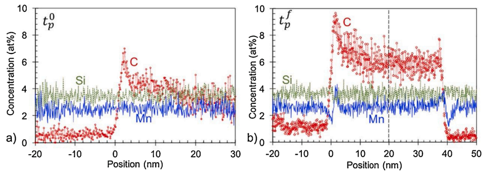
Fig. 19. Concentration profiles of C, Mn and Si in martensite and austenite for an Fe-0.3C-2.5 Mn-1.5Si (in wt.%) alloy during partitioning at 400 °C. (a) t_p^0 , at the beginning of the partitioning process. (b) t_p^f , after partitioning for 200 s [254].
