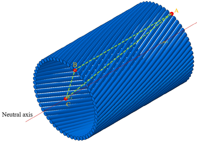
Fig. 4. Nodes involved in periodicity conditions on the helical components.
