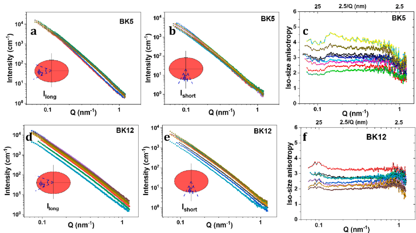
Fig. 9. Iso-size isotropy analysis of the organic-rich BK5 and BK12 shales and spatial heterogeneity in isosize anisotropy. (a, d) The scattering intensity I_{\text{long}} was obtained by sectorial radially averaging along the major axis of 2D SAXS profiles (inset) for different scan positions. (b, e) The scattering intensity I_{\text{short}} obtained by sectorial radially averaging along the minor axis of 2D SAXS profiles (inset) for different scan positions. (c, f) Q-variation of isosize anisotropy parameter \zeta at different scan positions.
