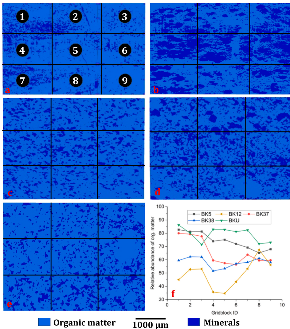
Fig. 5. Reconstructed and segmented X-ray CT image volume. (a-e) sequentially represent BK5, BK12, BK37, BK38 and BKU. The numbering scheme of grid units is shown in (a). (f) represents the relative abundance of organic matter (%) across different grid units.
