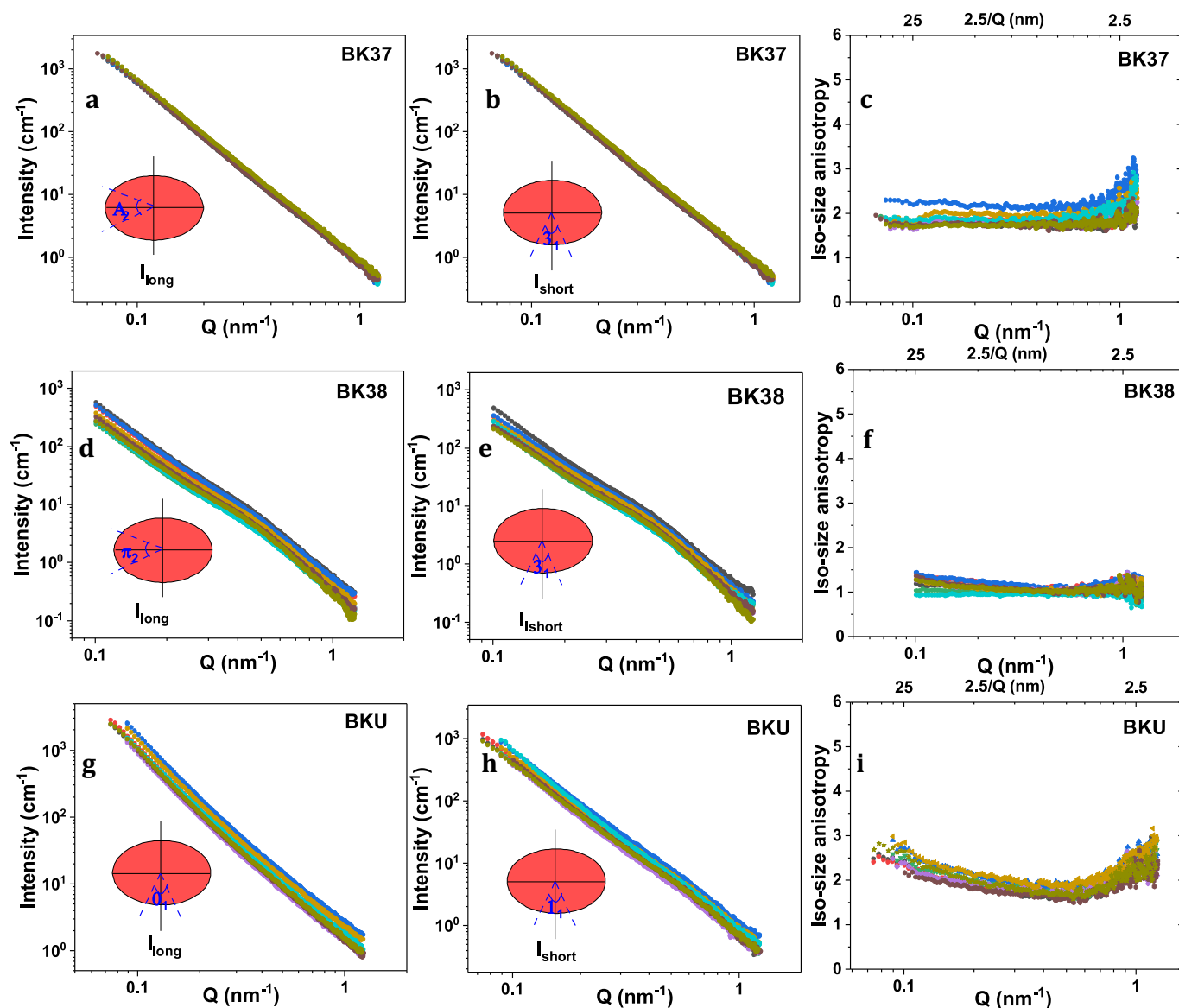
Fig. 10. Iso-size isotropy analysis of the organic-rich BK37, BK38, and BKU shales and spatial heterogeneity in isosize anisotropy. (a, d, g) The scattering intensity I_{\text{long}} was obtained by sectorial radially averaging along the major axis of 2D SAXS profiles (inset) for different scan positions. (b, e, h) The scattering intensity I_{\text{short}} obtained by sectorial radially averaging along the minor axis of 2D SAXS profiles (inset) for different scan positions. (c, f, i) Q-variation of isosize anisotropy parameter \zeta at different scan positions.
