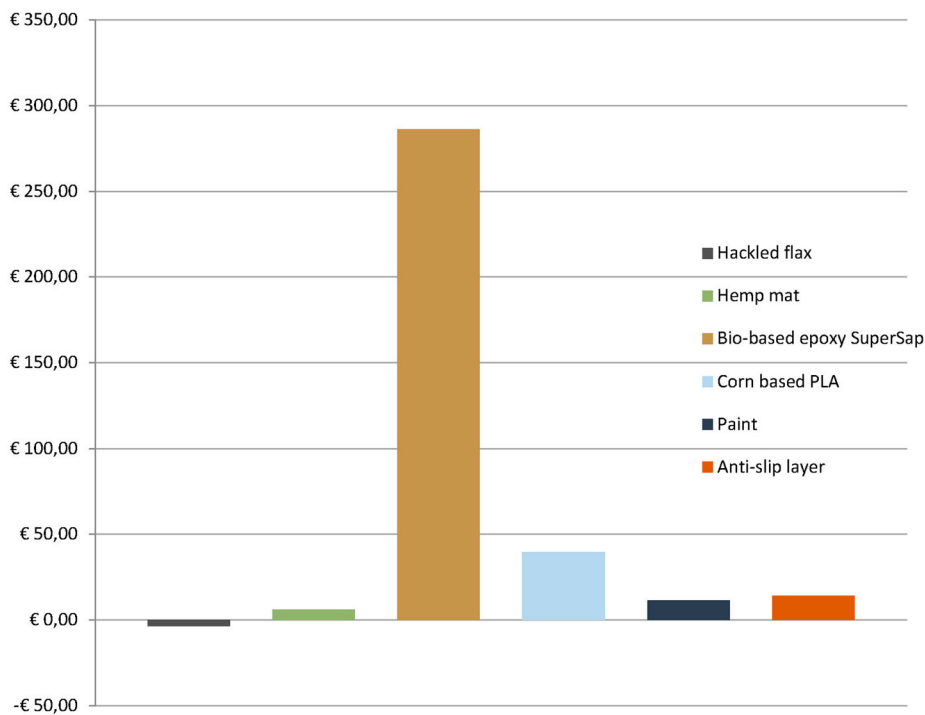
Fig. 29: Environmental cost impact for the total material used in to build the bridge
