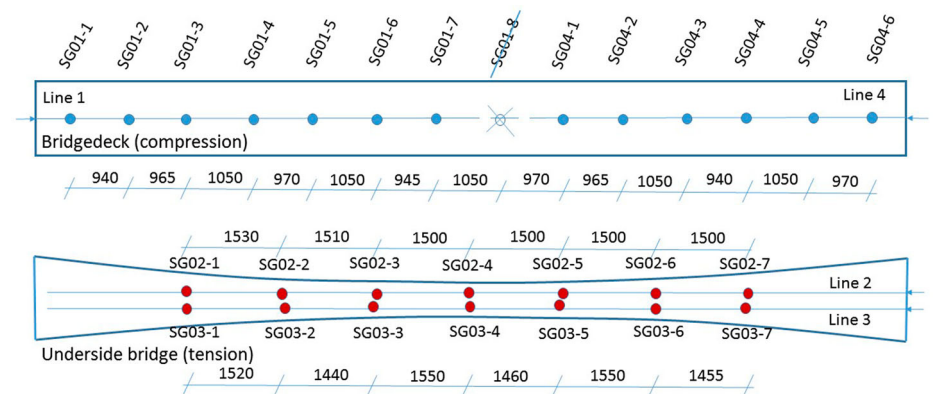
Fig. 10: Location of sensors. Line SG-01 and SG-04 are mainly compression (in bridge deck). Line SG-02 and SG-03 are mainly tension (underside bridge)
