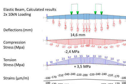
Fig. 27: Elastic model load test August 2018, calculated vertical deflections, the longitudinal compression and tension stresses and the strains
