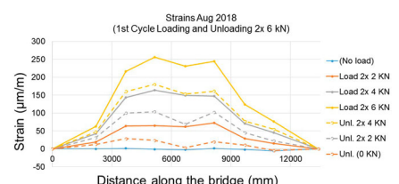
Fig. 23: First load cycle; results of strains in tension sensors along the bridge (line 2), loading and unloading to 2 \times 6.0 \text{ kN}
