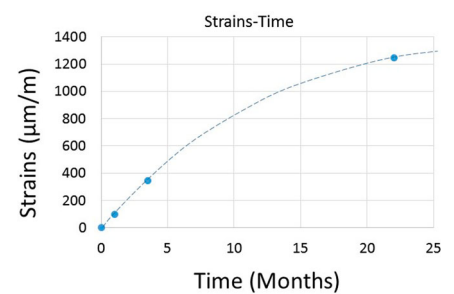
Fig. 28: Strain measurement results of unloaded bridge (only self-weight) of five measurements in time
