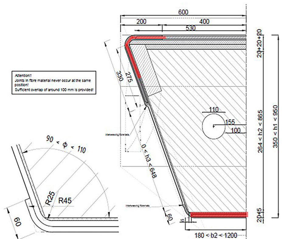
Fig. 13: Part of a production drawing, half of section in middle of the bridge, in red/dark is indicated the position the woven fibres
