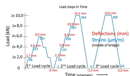
Fig. 22: Three load cycles during the test on 17 August 2018 showing applied load, max strain in middle and maximum measured vertical deflection
