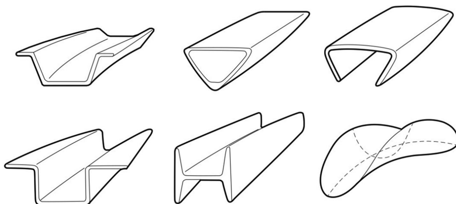
Fig. 2: Workshop output on variable bridge cross-sections
