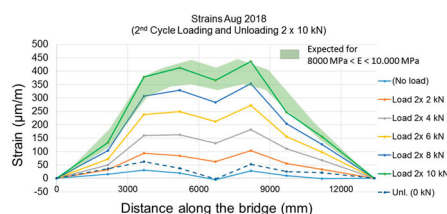
Fig. 24: Second load cycle; results of strains in tension sensors along the bridge (line 2), stepwise loading and unloading to 2 \times 10.0 \text{ kN}
