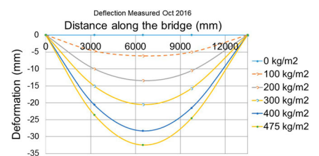
Fig. 17: Results measured LDVT deflections at production facility test 21 October 2016
