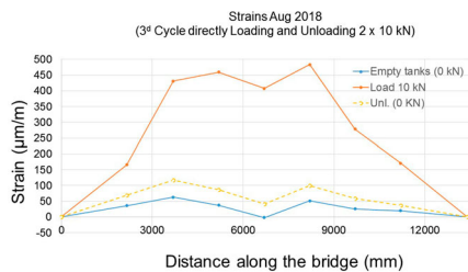
Fig. 25: Third load cycle; results of strains in tension sensors along the bridge (line 2), loading and unloading directly to 2x 10.0 kN. The dotted line shows the remaining strains
