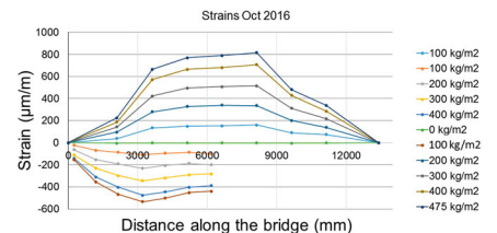
Fig. 18: Strain deformations as function of the applied load
