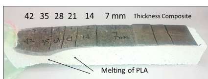
Fig. 12: Meltdown of the PLA foam occurred when the thickness of the lay-up exceeds 10 mm
