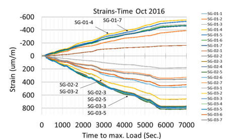
Fig. 19: Strain development versus time during loading; lines 2 and 3 are positive strains in tension (underside bridge beam) line 1 shows negative strains in compression (in bridge deck)
