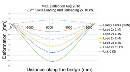
Fig. 26: Measured deflections (in middle of the bridge) during second loading (10 kN) and unloading cycle
