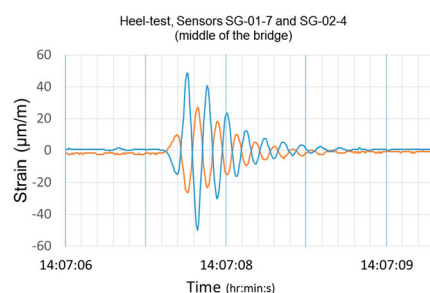
Fig. 20: Strain results versus time of sensors 1-7 and 2-4 showing Eigen frequency and damping
