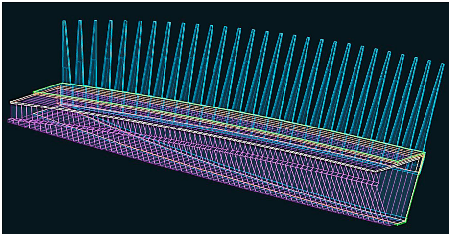
Fig. 11: Change in shape from rectangular to triangular using laser cut PLA foam elements
