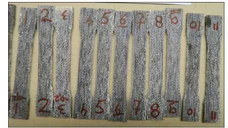
Fig. 5: Milled test samples from 1:1 model and tension test with optical strain measurement
