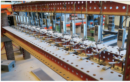
Fig. 7: Creep test set-up at TU/e laboratory
