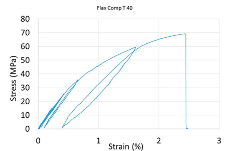
Fig. 6: Typical result of a repeated loading-unloading and reloading tension test in the laboratory on a test specimen of Woven (90 degrees) flax fibre composite showing hysteresis behaviour
