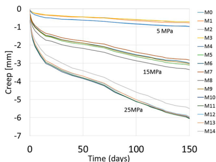
Fig. 8: Creep curves at three stress levels 5, 15 and 25 MPa in three-point bending tests
