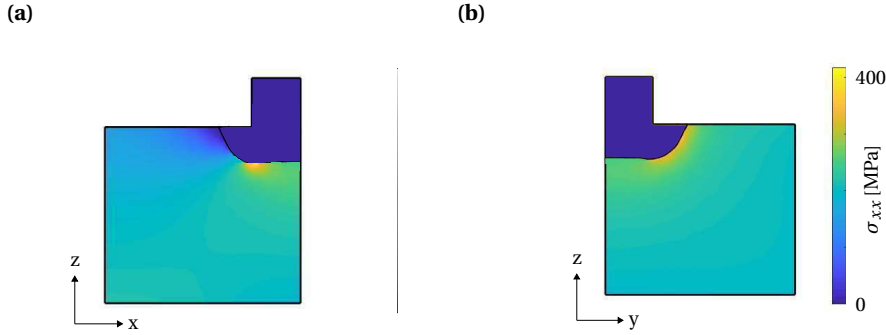
Figure 11: (a) The normal stress in the x-direction at the (a) XZ plane and (b) the YZ plane for a loaded specimen at maximum applied stress with a column height of 250 \mu\text{m} at 7200 seconds under a current density of 540 \mu\text{Amm}^{-2} .
