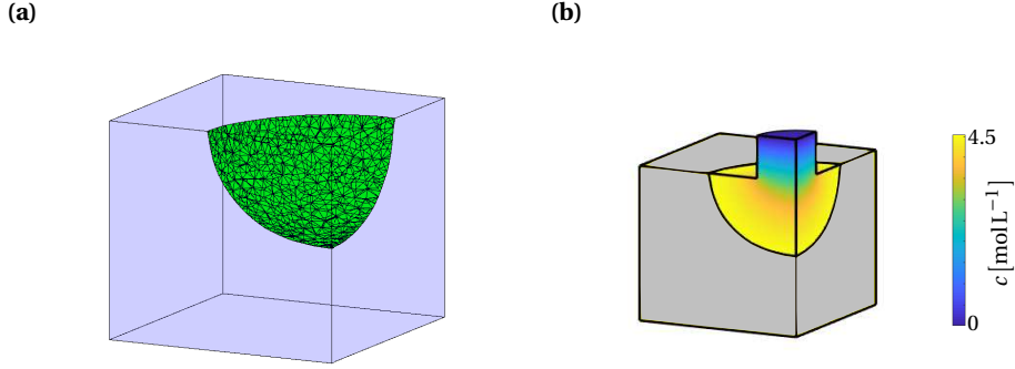
Figure 9: (a) The pit front shape and (b) the concentration distribution for a loaded specimen with a column height of 250\text{ }\mu\text{m} at 20400 seconds under a current density of 540\text{ }\mu\text{Amm}^{-2} .
