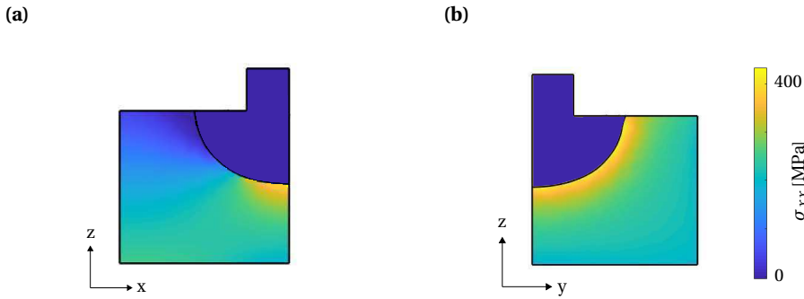
Figure 12: (a) The normal stress in the x-direction at the (a) XZ plane and (b) the YZ plane for a loaded specimen at maximum applied stress with a column height of 250 \mu\text{m} at 20400 seconds under a current density of 540 \mu\text{Amm}^{-2} .
