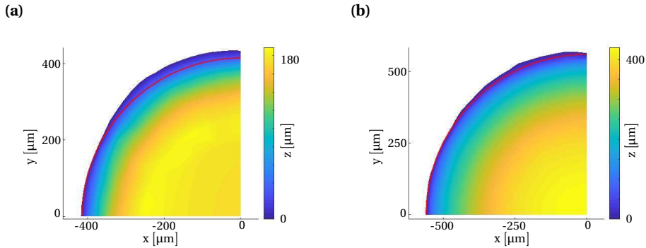
Figure 10: A pit depth map, excluding any mechanical deformation, at (a) 7200 and (b) 20400 seconds of the loaded specimen with a column height of 250\text{ }\mu\text{m} under a current density of 540\text{ }\mu\text{Amm}^{-2} . The red line indicates a perfect quarter of a circle.
