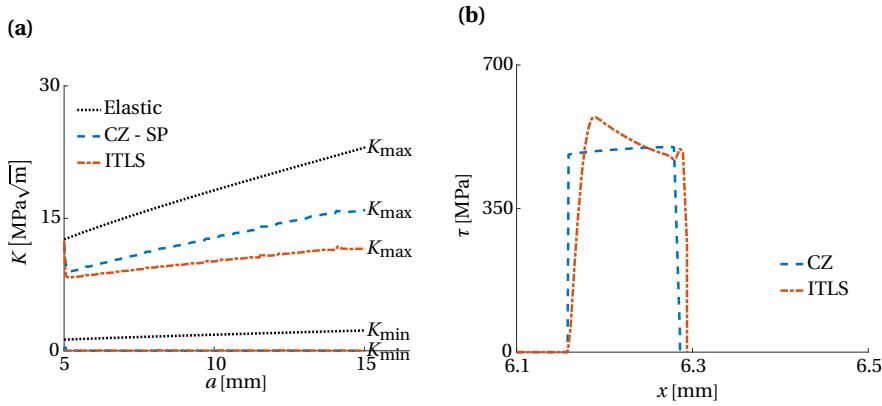
Figure 18: (a) The stress intensity factor versus crack length and (b) the fracture process zone cohesive traction distribution for the elastic-plastic centre crack specimen
