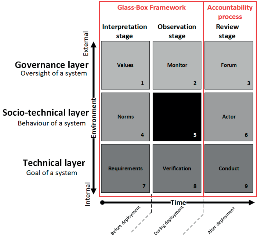
Figure 11: Glass Box framework projected on Comprehensive Human Oversight Framework
