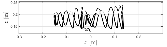
Fig. 9. Non-regular behaviour of the uncontrolled p-SLIP. The system is initialized with \alpha(0) = 0.2 \text{ rad} , r(0) = 0.144 \text{ m} , \dot{\alpha}(0) = \dot{r}(0) = 0 , and a constant attack angle = 0.2 \text{ rad} . The trajectory of the CoM is depicted with solid lines during stance and with dotted lines during flight.
