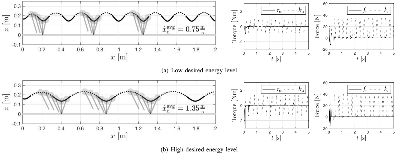
Fig. 11. Simulations of the p-SLIP controlled using the proposed approach showing stable forward hopping for two energy levels. For both simulations, the system is initialized with \alpha(0) = 0.2 \text{ rad} , r(0) = 0.19 \text{ m} , \dot{\alpha}(0) = \dot{r}(0) = 0 . Control inputs for each simulation are also reported, together with the corresponding spring contributions. After few steps, the motion evolves along the nonlinear mode, and the control action converges to zero.
