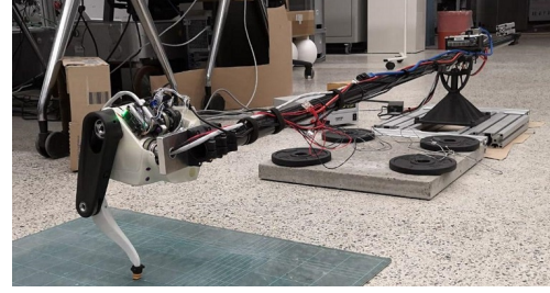
Fig. 12. Experimental setup used to validate the strategy proposed in this paper. An elastically actuated articulated leg is connected to a pole hinged at a point. The pole constrains the rotation of the trunk body, thereby forcing the system to evolve along the sagittal plane with free translation and fixed rotation of the trunk.
