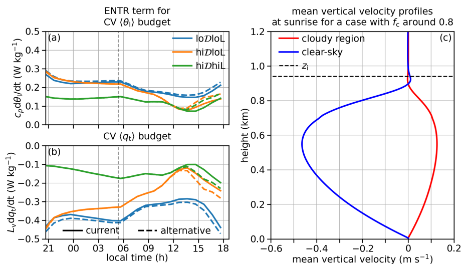
Figure 13. Time series of current and alternative estimates of the entrainment contribution to CV (a) \langle \theta_1 \rangle and (b) \langle q_t \rangle budgets. The vertical dashed black lines indicate sunrise. Panel (c) shows an example to facilitate the discussions near the end of Sect. 6.1.
