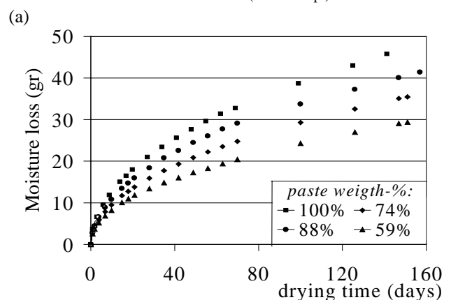
Figure 5. Moisture loss as a function time, (a) numerical analysis, (b) experimental results (Bisschop & Van Mier 2001).
