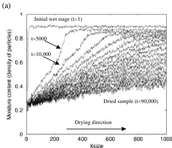
Figure 4. Density profiles due to drying at different time steps for (a) r = 1 , (b) r = 0 .
