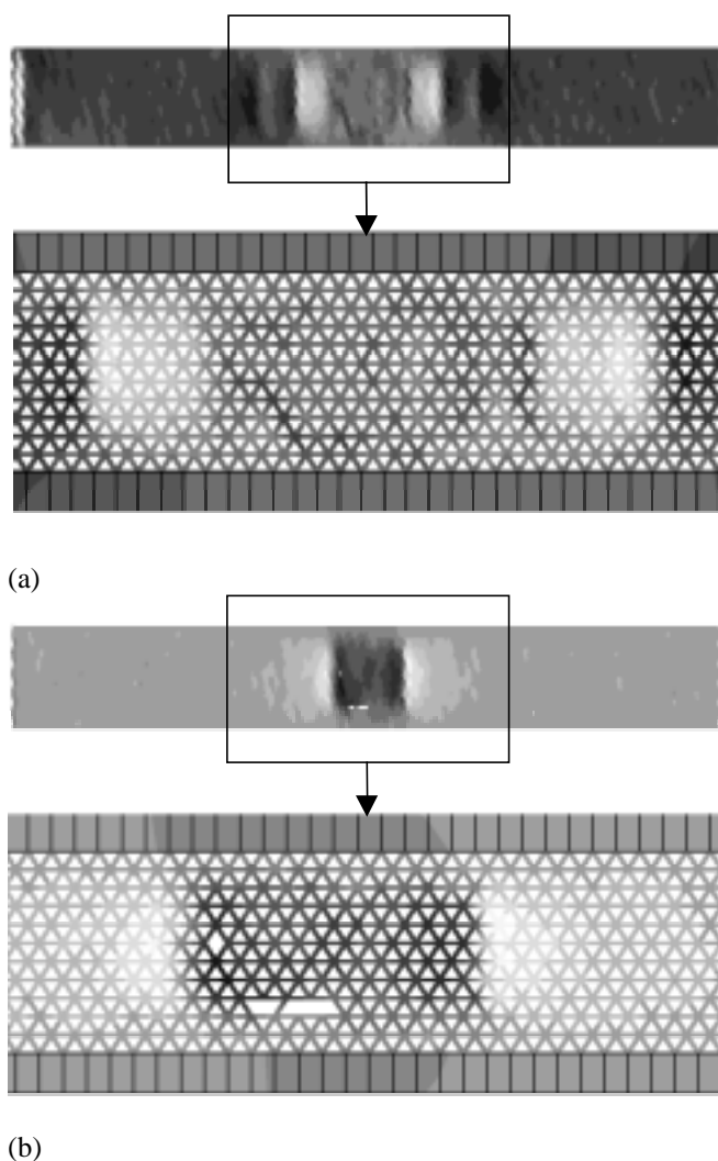
Figure 11. Deformations and cracks in LFM, (a) after 1000 steps in LGA, r = 0 , (b) after 15,000 steps in LGA, r = 0 .
