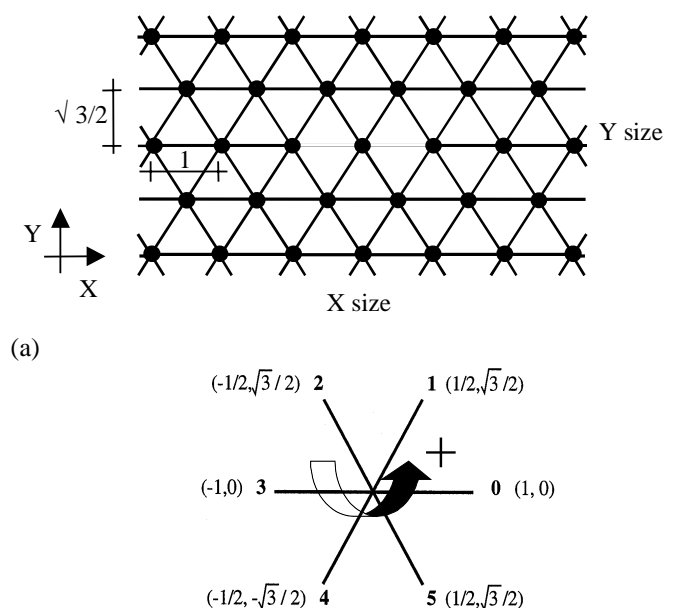
Figure 1. (a) Lattice Gas Automaton, FHP model, (b) movement of the particles with velocities ( c_i ) in six directions.
