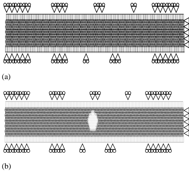
Figure 9. Lattice Fracture Model: mesh with the supports (continuum elements supported on top/bottom), (a) homogeneous structure (b) with single aggregate in the middle.
