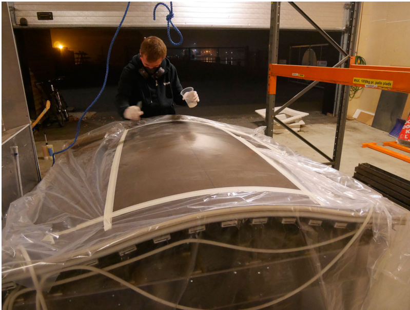
Figure 15. Setting out of the tested mould shape on the flexible table and adding the first layers, panels size 1 × 0.5 m.
