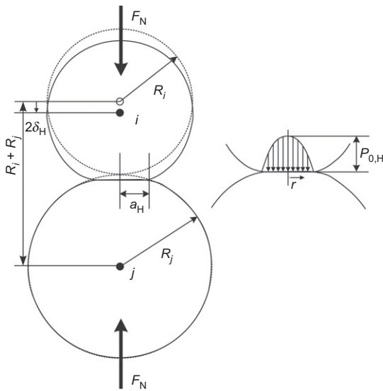
Fig. 8. Schematic drawing of two spherical grains subjected to a compressive load F_N , modified from Caicedo (2018)
