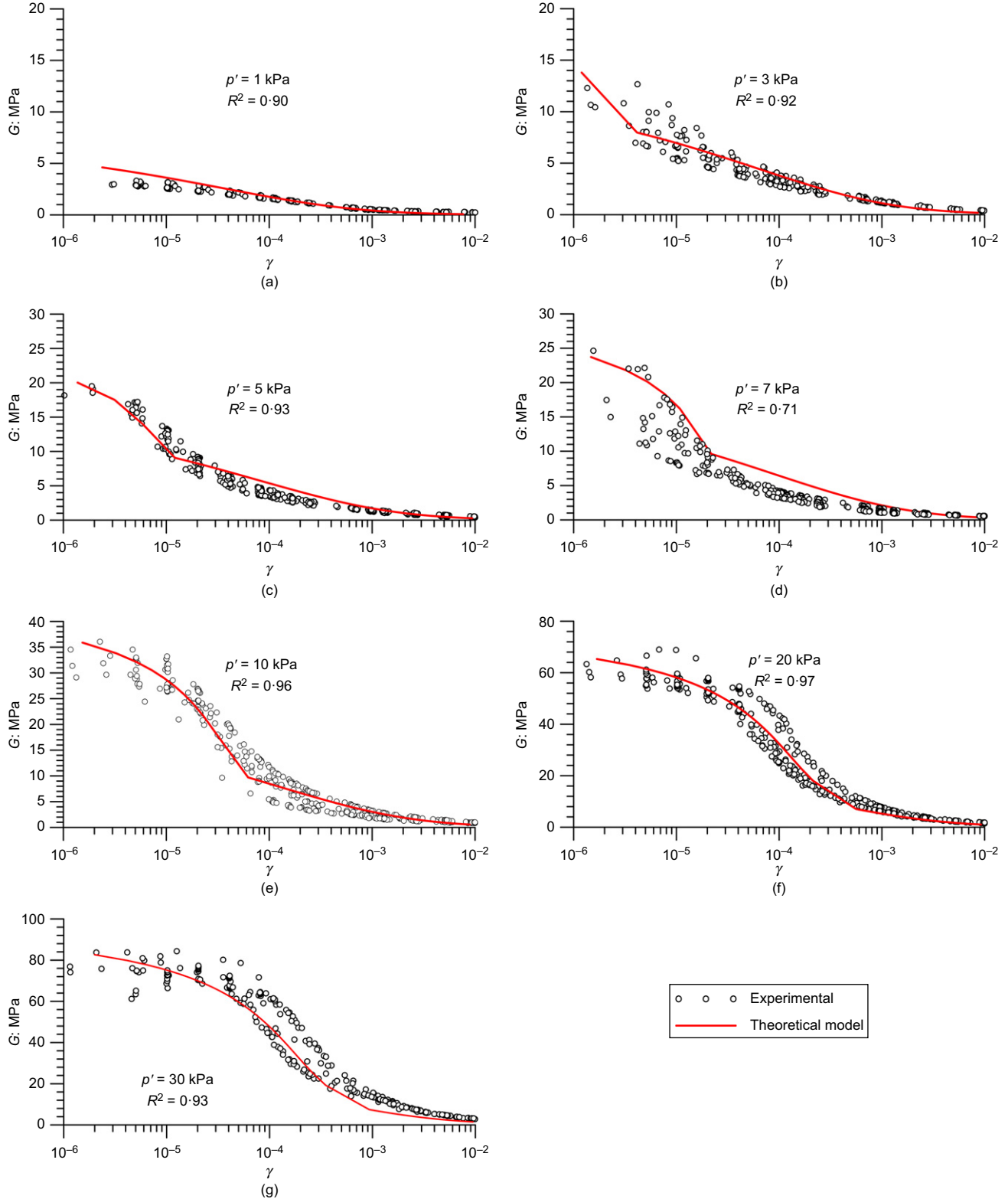
Fig. 14. Comparison between the experimental results of shear modulus (see section ‘Experimental work’) and the predictions of the theoretical model (see section ‘Performance of the micromechanical model for the whole range of confining stresses’) for the whole range of confining stresses. The parameters of the model are shown in Table 1
