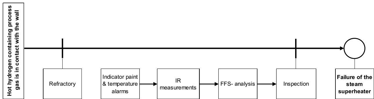
Fig. 7. Left part of the bowtie regarding creep and Nelson hydrogen attack of the steam superheater (IR: infrared; FFS: fitness for service).
