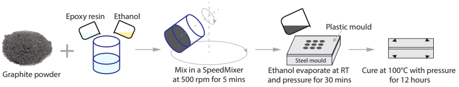
Figure 3.6: The schematic of composite fabrication process.
