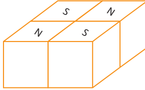
Figure 4.8: An array of four permanent magnets with alternating magnetic poles, where 'N' represents the north pole and 'S' the south pole, respectively.
