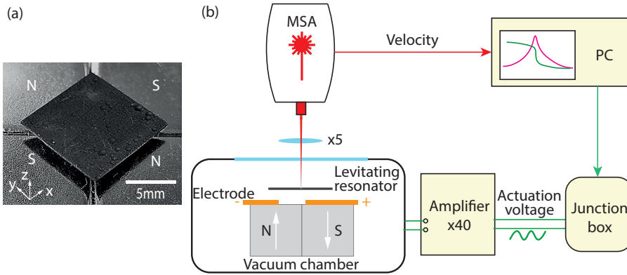
Figure 2.1: The levitating resonator and experimental setup. (a) Levitating pyrolytic graphite plate above 4 cubic Nickel coated NdFeB magnets with alternating magnetization, where N and S stand for north and south pole of the magnet, respectively. The origin of the coordinate system is at the center of the plate. (b) Schematic of the measurement setup comprising a MSA400 Polytec LDV for the read out and electrostatic excitation method. The actuation voltage is generated by the LDV junction box and is amplified by a 40 \times voltage amplifier that drives the levitating plate into resonance using electrostatic actuation. The electrostatic force is generated via two electrodes beneath the levitating plate. By focusing MSA laser beam on the plate, the vibration signal is detected, and the acquired velocity is transferred to a PC for frequency response analysis.
