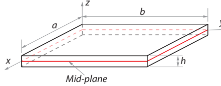
Figure 5.7: Geometry of the rectangle plate and coordinate system
