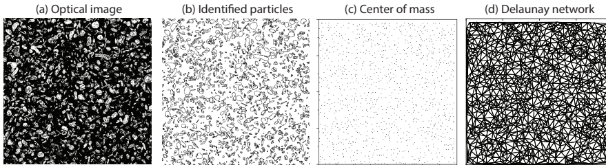
Figure 3.9: Particle dispersion analysis on a composite with 17.6\ \mu\text{m} particles and 20.8 % volume fraction. To obtain the Area Disorder AD , we first take an image of the composite (a) and then identify the particles (b) using ImageJ. Afterwards, the particles' center of mass (c) is located, from which we build their Delaunay network (d) to calculate the AD .
