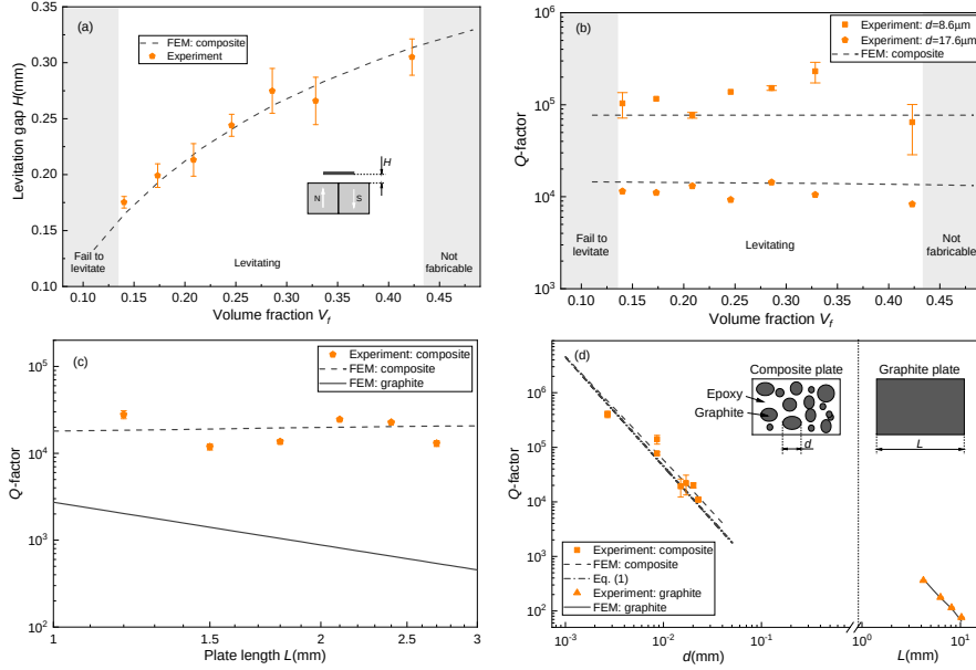
Figure 3.4: Dependence of the levitation force and dissipation on composite particle and plate size. (a) Levitation gap H of the 1.8 \times 1.8 \times 0.09 \text{ mm}^3 plate with 17.6 \mu\text{m} particles as a function of volume fraction. (b) Q-factor of two 1.8 \times 1.8 \times 0.09 \text{ mm}^3 plates with different particle size as a function of volume fraction. The gray area in Fig. 3.4a-b represents the volume fraction of which the composites can not be levitated. (c) Q-factor of square composite plates with a thickness of 90 \mu\text{m} as a function of plate side length L . The composite plates are made from d = 17.6 \mu\text{m} particles with 0.21 volume fraction. (d) Dependence of Q on particle size. The left side of the graph (before the short dashed line) shows the Q of composite plates with varying graphite particle size. Since the Q is only weakly dependent on the volume fraction and side length (see Fig. 3.4b-c), the error bars in the data on the left side of Fig. 3.4d are obtained by analyzing the Q s obtained from plates with a thickness of 90 \mu\text{m} but different side lengths (1.2-2.7 mm) and volume fraction (0.14-0.32) at fixed d . The right side of the graph (after the short dashed line) shows the experimental Q of levitating plates made of pyrolytic graphite with 0.28 mm thickness and different side lengths L on the x-axis. The insets show schematics of the composite and graphite plate. In Fig. 3.4, the dashed and solid lines correspond to the FEM simulations for composite and graphite plates as described in A3, respectively. Moreover, the dashed-dotted line in Fig. 3.4d represents the Q s obtained from Eq. (3.1). The dots represent experimental data.
