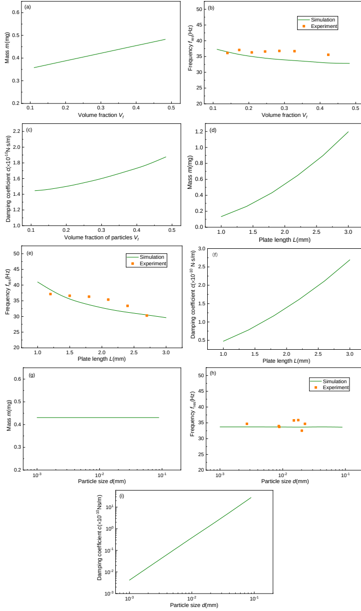
Figure 3.14: (a-c) Changes in mass m , resonance frequency f_{res} and damping coefficient c of 1.8 \times 1.8 \times 0.09 \text{ mm}^3 composite plates with d=17.6 \mu\text{m} particles and different volume fraction V_f ; (d-f) Changes in mass m , resonance frequency f_{res} and damping coefficient c of composite plates with d=17.6 \mu\text{m} particles and volume fraction V_f = 0.21 , but different plate length L ; (g-i) Changes in mass m , resonance frequency f_{res} and damping coefficient c of 1.8 \times 1.8 \times 0.09 \text{ mm}^3 composite plates with volume fraction V_f = 0.32 and different particle size d . The lines correspond to data obtained from COMSOL simulations and dots represent measured data.
