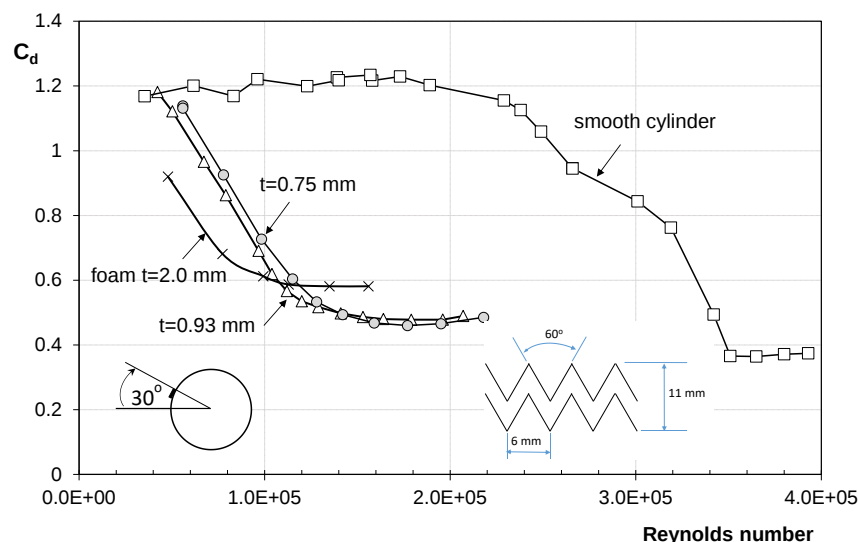
Figure 5. The effect of zigzag tape thickness on the drag coefficient of a cylinder. Tape at an azimuth position of 30^\circ on the left and right from the leading edge. Cylinder span is 60 cm. If not indicated otherwise, the zigzag tape used during all measurements has the layout of the Teflon tape shown in the insert.
