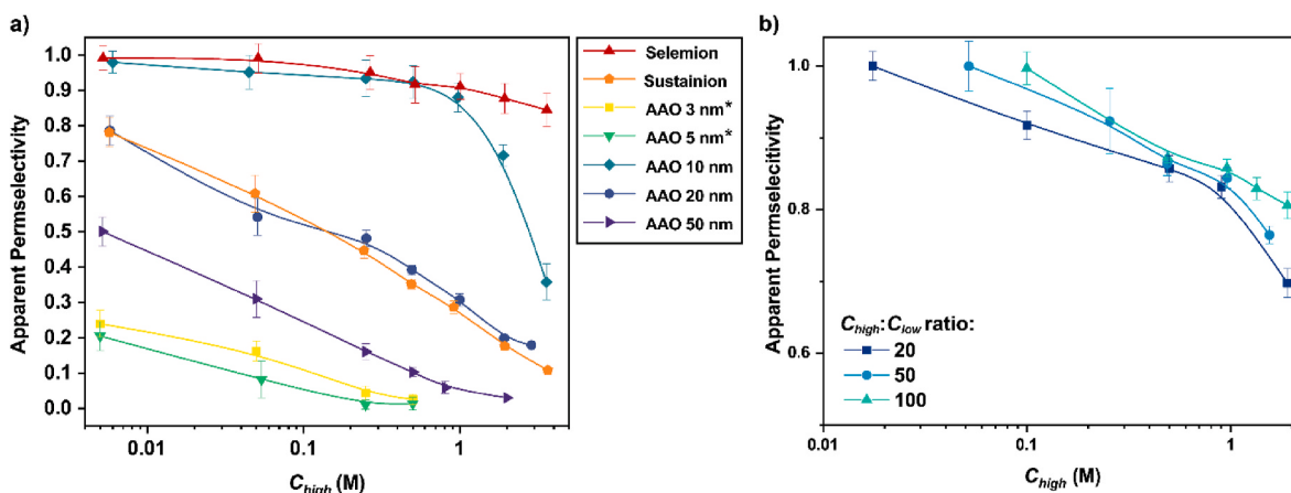
Fig. 2. a) Apparent permselectivity of two polymeric IEMs – Selemon AMV and Sustanion X37 – and five AAO membranes with different pore sizes (3–50 nm) placed between two reservoirs with a concentration ratio of 5.*3-nm and 5-nm pores are asymmetric membranes with only a thin selective layer. b) Apparent permselectivity results showcase the effect of concentration and concentration ratio on permselectivity of the AAO membrane with 10-nm pores. Note that the figures have different scales.
