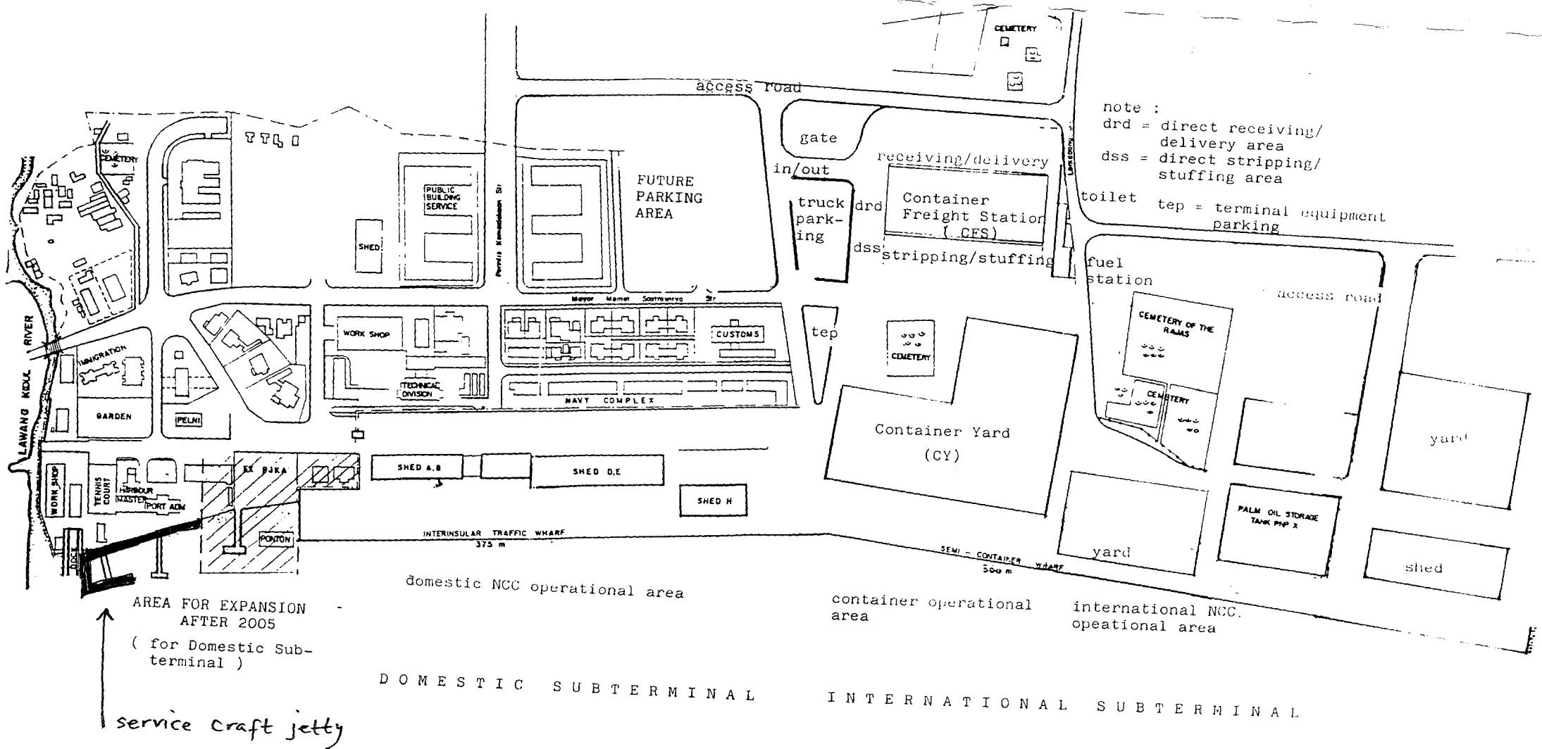
figure 4.3 THE 2005 MPT LAYOUT
