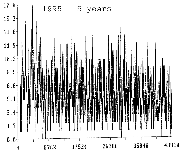
figure 3.3.a Cycle length of 1986 1990 1995 and 2005 situation.
