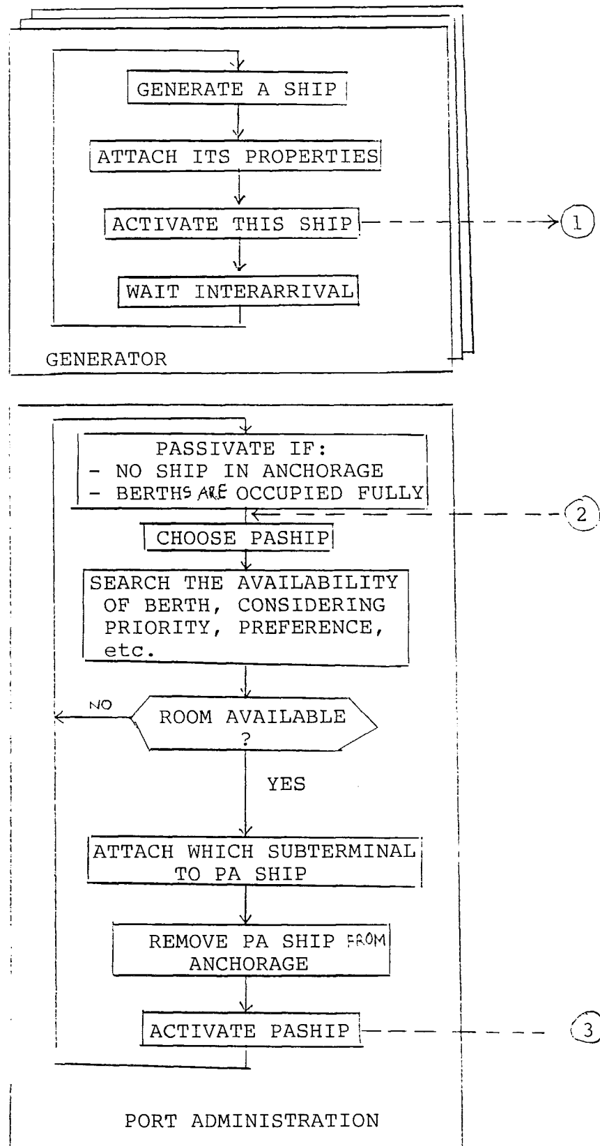
figure 3.2. Flowchart of the MPTSIM program
