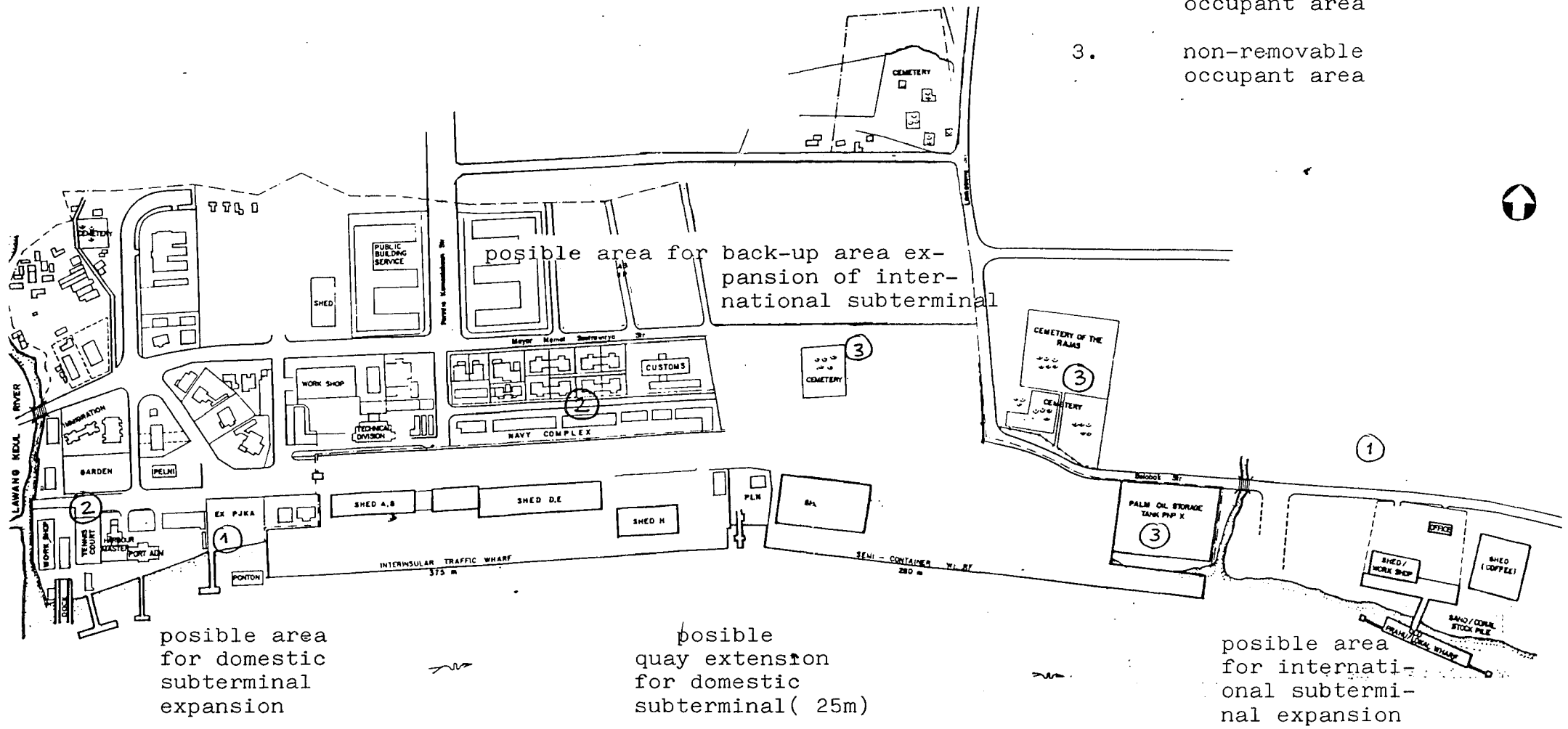
figure 4.1 The likely MPT layout in 1990 and the possible expandable area of its surroundings.
