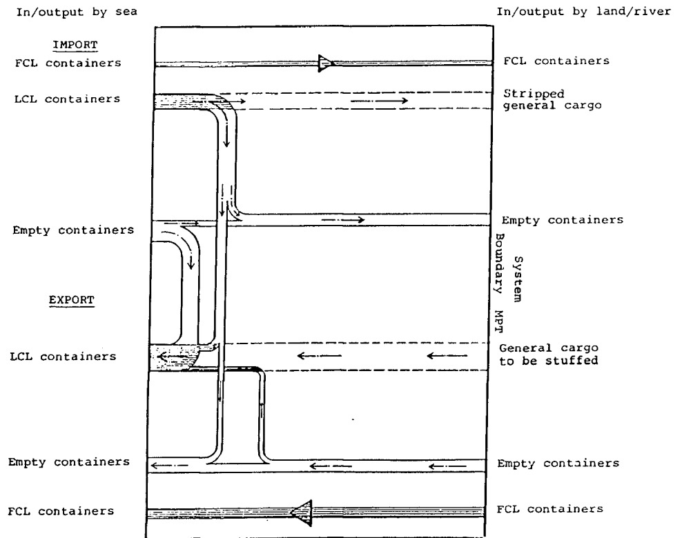
figure C2.2 Qualitative container flow
