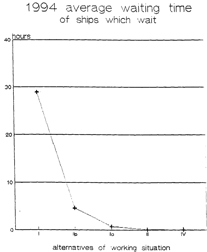
figure 3.8 The 1994 Port Operation Indicators (when the international quay of 100 m being rebuilt )
