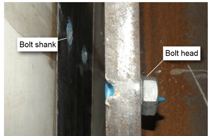
Fig. 19. Sheared bolt after failure (P15.2-1).
