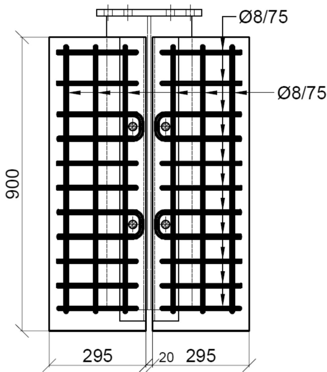
Fig. 5. Reinforcement layout.
