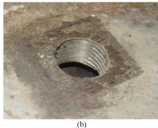
Fig. 17. Observed damages (P15.1-1) (a) sheared bolt and (b) thread penetration.
