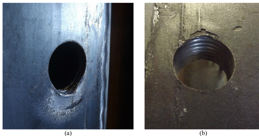
Fig. 12. Observed damages (P3.1-1) (a) bearing deformation and (b) thread penetration in the steel beam.
