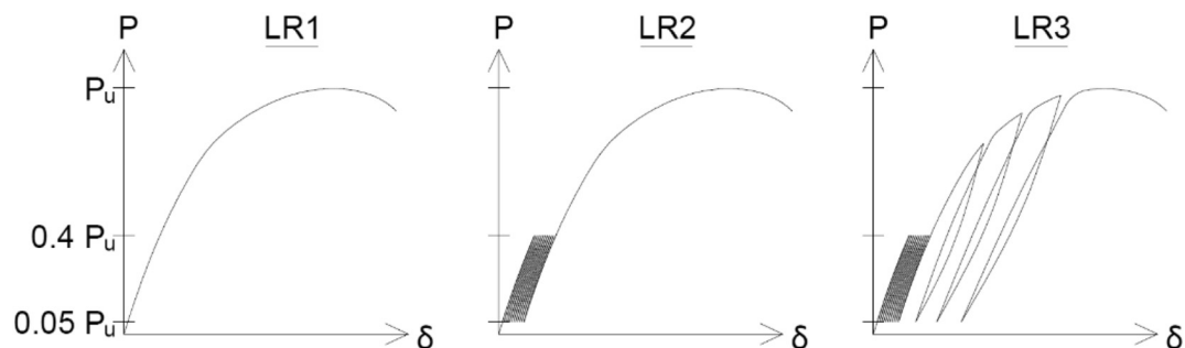
Fig. 10. Loading regime.
