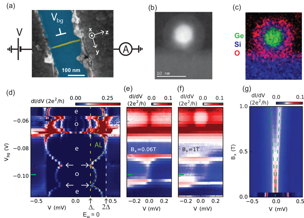
Figure 1. (a) False colored scanning electron microscope image of the device with the NW (yellow) with aluminum contacts (gray) on a Si/SiN x wafer (blue). The magnetic field axes, voltage bias measurement setup, and global bottom gate are indicated. (b) Transmission electron microscope (TEM) image of the cross section of the NW. (c) Energy dispersive X-ray spectroscopy of the area displayed in panel b. The colors represent different elements: Ge is green, Si is blue, and oxygen (O) is red, respectively. The Ge–Si core–shell wire is capped by a SiO x shell. (d) Voltage bias tunneling spectroscopy measurement of the superconducting quantum dot as the bottom gate voltage V_{bg} is altered. The superconducting gap, an Andreev level (AL), and multiple Andreev reflections appear as peaks in differential conductance ( dI/dV ). The AL, \Delta , and 2\Delta are marked by dashed green, yellow, and white lines, respectively. The even or odd occupation is indicated, and the kink in the observed Andreev level is highlighted by the arrows. (e, f) Same measurement as panel d with a magnetic field, B , applied perpendicular to the substrate ( x -direction) of 60 mT and 1 T, respectively. A zero bias Kondo peak is observed as the quantum dot is occupied by an odd number of electrons. At B = 1 T, the resonance is split due to the Zeeman effect. (g) Linear splitting of the Kondo peak at V_{bg} = -0.098 V as a function of B . The Zeeman effect splits the spinful Kondo peak, which is indicated by the dashed green line.
