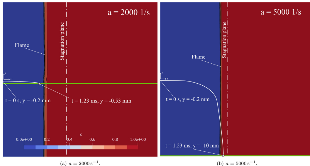
Fig. 4 – Streamlines intersecting the left boundary at vertical coordinate y = -0.2 \text{ mm} for two applied strain rates a are plotted on top of water mass fraction based normalised progress variable contours. Green lines indicate the section along with the integral of NO is computed for the two cases after the same travelling time t = 1.23 \text{ ms} .
