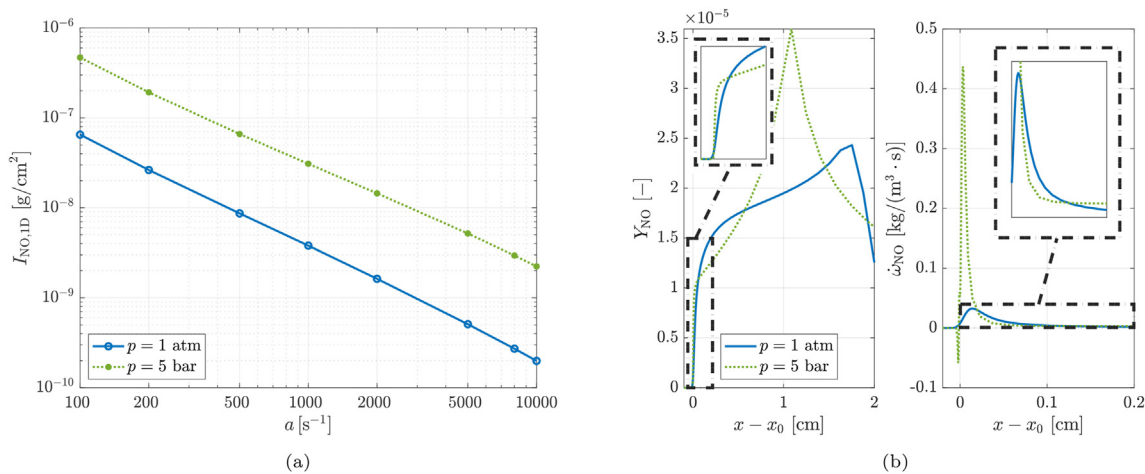
Fig. 9 – (a) Variation of density weighted NO integral I_{NO} with strain a for a hydrogen-air flamelet at \varphi = 0.7 at p = 1 atm and p = 5 bar. (b) Distribution of NO mass fraction Y_{NO} and NO source term \dot{\omega}_{NO} across the flamelets for the two pressure conditions for a = 500 s -1 . The regions indicated by the dashed rectangle are zoomed out for clarity.
