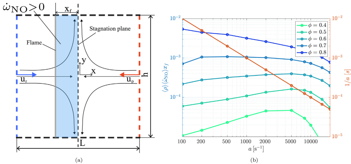
Fig. 11 – (a) Control volume around the counter-flow premixed reactants-to-products flame configuration used for the analytical derivation of the correlation for I_{NO} . (b) Variation with strain a of the numerator of Eq. (24) for the hydrogen-air premixed flame at different equivalence ratios \phi , as compared to the function 1/a .
