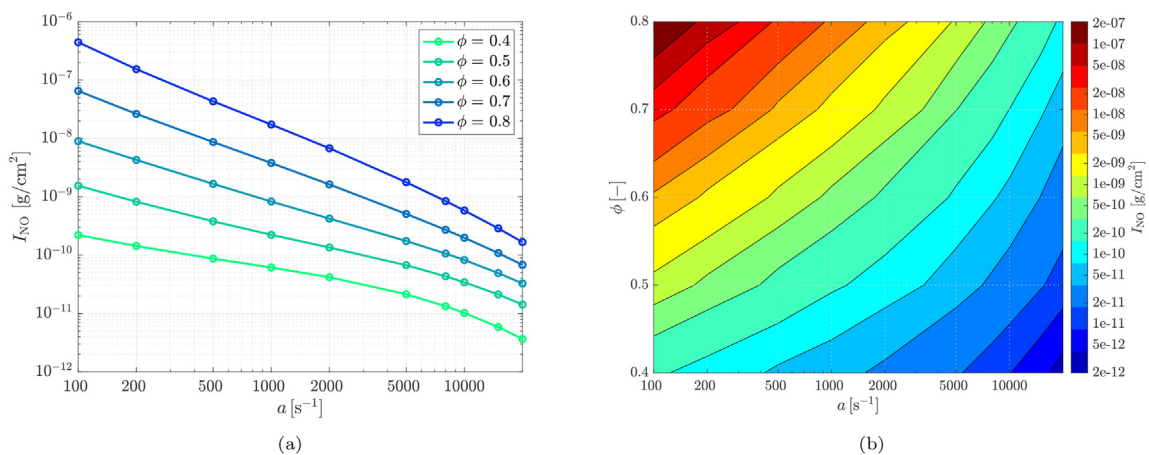
Fig. 10 – (a) Variation of density weighted NO integral I_{\text{NO}} with strain a for hydrogen-air flame at different equivalence ratios \phi . (b) Contour plot of density weighted NO integral I_{\text{NO}} as a function of strain a and equivalence ratio \phi .
