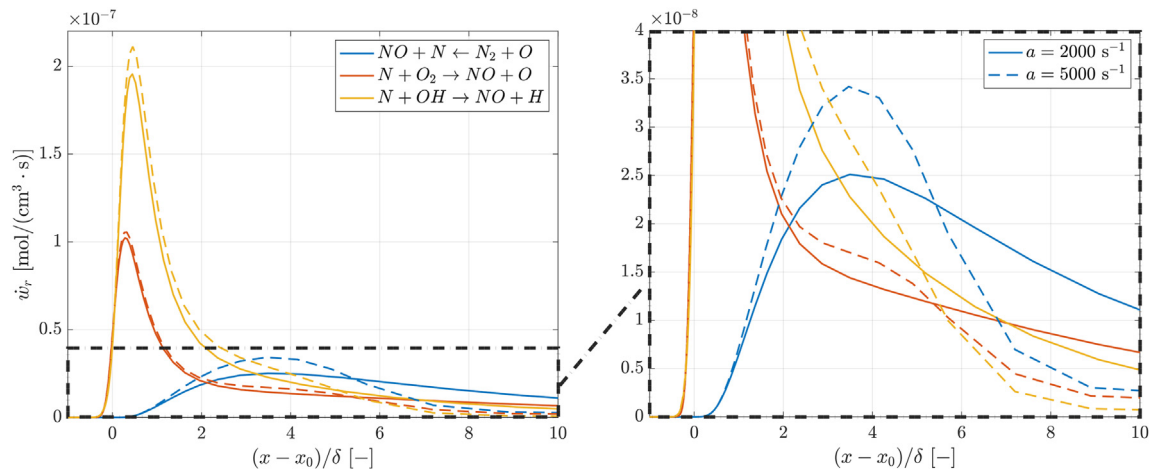
Fig. 7 – Molar rate of thermal NO x reactions \dot{w}_r across a hydrogen-air flamelet at equivalence ratio \phi = 0.7 , for two applied strain rates of a = 2000 \text{ s}^{-1} (solid line) and a = 5000 \text{ s}^{-1} (dashed line). A zoom in the region indicated by the dashed rectangular area is shown on the right for clarity.
