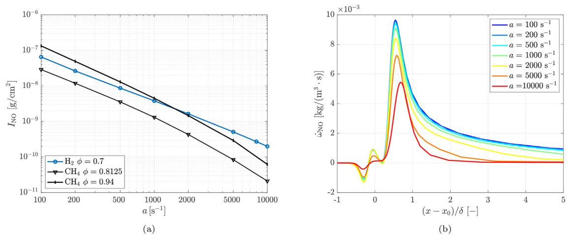
Fig. 8 – (a) Variation of density weighted NO integral I_{NO} with strain a for a methane-air flamelets at two equivalence ratios and hydrogen-air flamelet at \phi = 0.7 . (b) NO source term \dot{\omega}_{NO} across the flamelet for different strain rates for methane at \phi = 0.8125 (same adiabatic flame temperature as hydrogen at \phi = 0.7 ).
