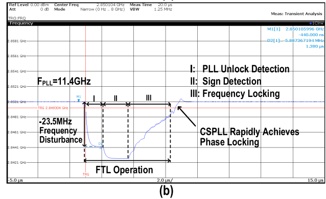
Fig. 18. Measured FTL transient response to (a) positive frequency disturbance and (b) negative frequency disturbance.
