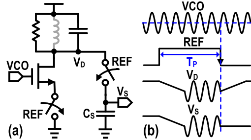
Fig. 1. (a) Schematic and (b) conceptual waveforms of a voltage-sampling PD using a power-gated isolation buffer.
