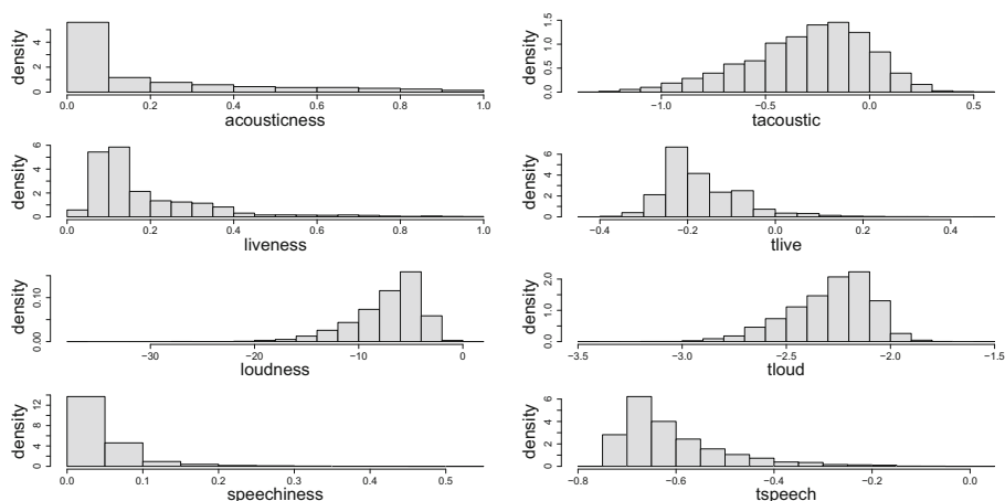
Fig. 2 Histogram of acoustiness (left), liveness (left), speechiness (left), loudness (left), and transformed acoustiness (right), transformed liveness (right), transformed speechiness (right) using the logit transform and transformed loudness (right) using the cube root transform in Rock
