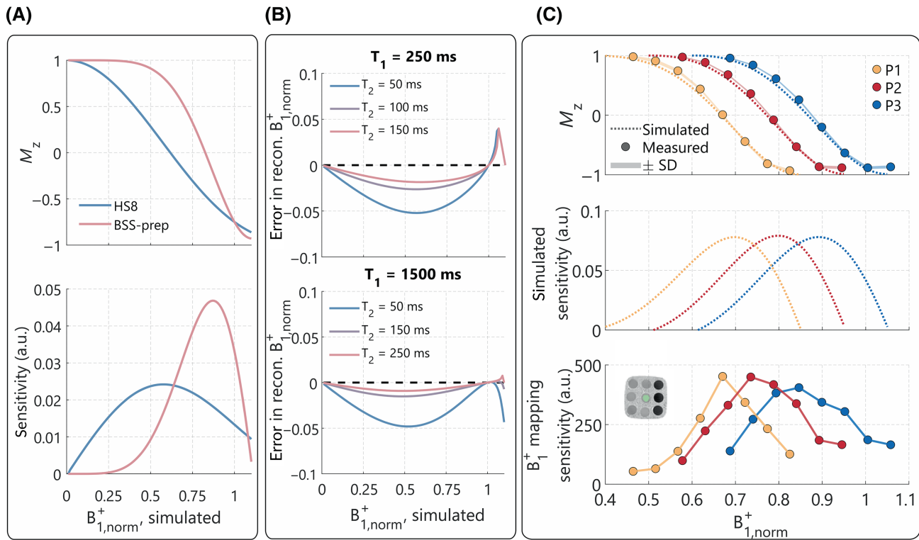
FIGURE 2 (A) Bloch-simulations of |B_1^+| sensitizing preparations based on Bloch-Siebert shift (BSS), with d_{BS} = 4.6 ms Fermi pulses, 13.5 \mu\text{T} amplitude, and tip-back phase \phi_{TB} = 0 (red) and su-adiabatic hyperbolic-secant 8 (blue). The top panel shows the postpreparation magnetization as a function of the |B_1^+| strength and the bottom panel shows the sensitivity, defined as the derivative of the postpreparation magnetization with respect to B_{1,norm}^+ . Increased sensitivity is observed with BSS-based preparations for higher |B_1^+| magnitudes ( |B_1^+| > 0.64 ). (B) B_1^+ map reconstruction bias due to relaxation effects for various T_2 times in the presence of a short T_1 (top) and long T_1 (bottom). Small underestimation of less than 0.05 is observed, with the largest deviation occurring for B_{1,norm}^+ > 1.0 or B_{1,norm}^+ \approx 0.5 . (C) B_1^+ mapping performance of three different preparations (P1, P2, and P3). The preparation parameters were tailored for different peak sensitivities, with Fermi pulse duration d_{BS} = 10/9/8 ms, tip-back phase \phi_{TB} = -40^\circ / -70^\circ / -90^\circ , and tip angle of 110^\circ/100^\circ/90^\circ , respectively. Postpreparation magnetization M_{4\phi}/M_{0\phi} (top plot) shows good agreement between simulated data (dashed lines) and phantom (solid line). Mapping sensitivity in simulations (middle plot) and experiments (bottom panel) show comparable trends with a shift in peak sensitivity to higher B_1^+ values from P1 to P3. The phantom region of interest in the central vial is indicated in the bottom panel. (A) Mapping sensitivity; (B) Relaxation-induced error; (C) Preparation tailoring.
