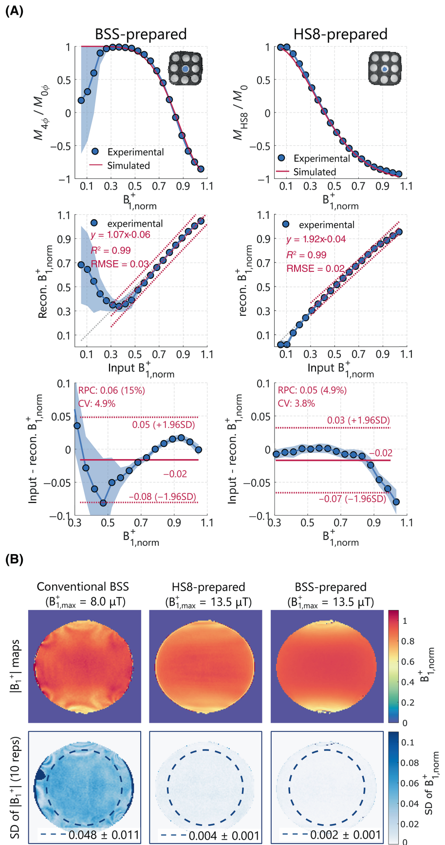
FIGURE 3 (A) Overlay of simulation and phantom results of the |B_{1+}| dependent signal using the proposed Bloch–Siegert shift (BSS)-preparation (left) with d_{BS} = 4.6 ms Fermi pulse duration, B_{1+,max} = 13.5 \mu T and \phi_{TB} = 0 , and the hyperbolic-secant 8 (HS8)-sensitization (right). The top plots illustrate postpreparation longitudinal magnetization ratio M_{4\phi}/M_{0\phi} and M_{HS8}/M_0 , while the middle plots show radiofrequency (RF) scaling and reconstructed B_{1+} linearity (left and) and bottom—the corresponding Bland–Altman analysis. (B) B_{1+} maps in the cylindrical phantom obtained using the conventional BSS mapping sequence (top left), the HS8-sensitization (top middle) and the proposed BSS-prepared method (top right). The corresponding SD maps from ten measurements are illustrated in the bottom row, with mean values over the region of interest (dashed line) of 0.048 \pm 0.007 for the conventional BSS, 0.046 \pm 0.001 for the HS8-sensitization, and 0.002 \pm 0.001 for the proposed method. (A) RF scaling in T1MES phantom; (B) |B_{1+}| and SD maps.
