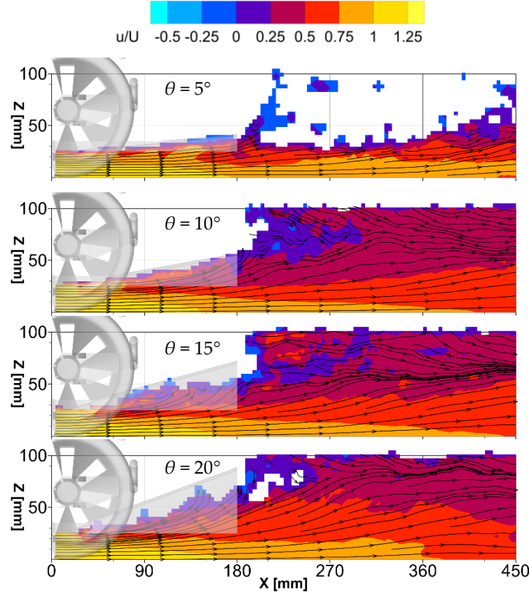
Figure 9. Contours of the streamwise velocity component with streamlines in the diffuser region at the car's symmetry plane ( Y = 0 ) for the four diffuser angles (from top to bottom: \theta = 5^\circ , 10^\circ , 15^\circ and 20^\circ ).
