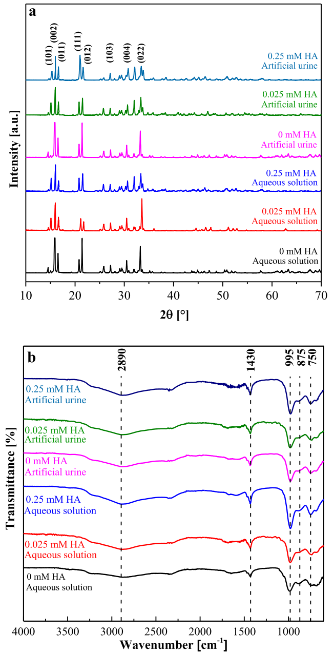
Fig. 1. a) X-ray diffraction (XRD) results and b) Fourier transform infrared (FTIR) results for the struvite crystals obtained in aqueous solution and artificial urine using different concentrations of hyaluronic acid (HA).
