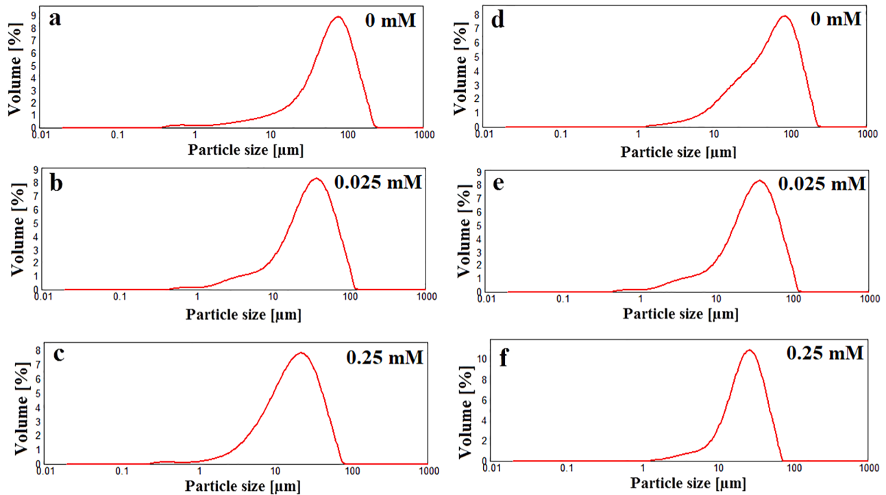
Fig. 3. Particle size distributions of the struvite crystals obtained in a) aqueous solution with 0 mM, b) 0.025 mM, and c) 0.25 mM hyaluronic acid and in d) artificial urine media with 0 mM, e) 0.025 mM, and f) 0.25 mM hyaluronic acid.
