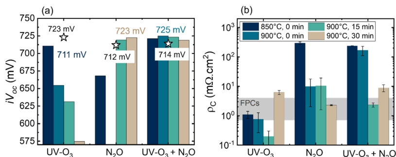
Figure 4. Implied V_{oc} ( iV_{oc} ) after hydrogenation (a) and contact resistivity (b) results for layers featuring a UV-O 3 , N 2 O and a combination of both oxides and annealed in a tube furnace with different annealing temperature and dwell times. The iV_{oc} data point relative to the N 2 O oxide with 900 °C, 0 min annealing is missing due to a damaged sample. To facilitate comparison with the RTP annealed samples, in (a), the best results obtained with RTP on each oxide type are indicated by the white stars (for optimized conditions). In (b), the typical range of contact resistivities achieved with optimized RTP conditions is highlighted by the gray-shaded area. The error bars denote the standard deviation over 2 or 3 different samples.
