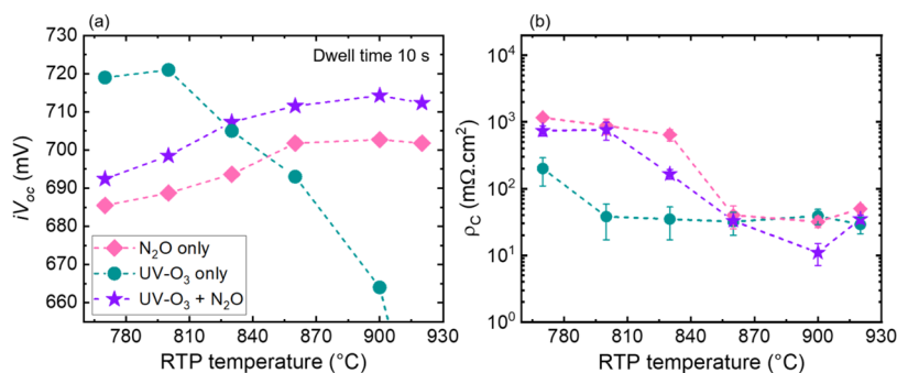
Figure 3. Implied V_{oc} ( iV_{oc} ) values after hydrogenation (a) and contact resistivity results (b) for N 2 O only (pink diamonds), UV-O 3 only (green circles) and UV-O 3 + N 2 O (purple stars) as a function of RTP temperature, for dwell times of 10 s. The error bars in (b) denote the standard deviation over 4 different samples.
