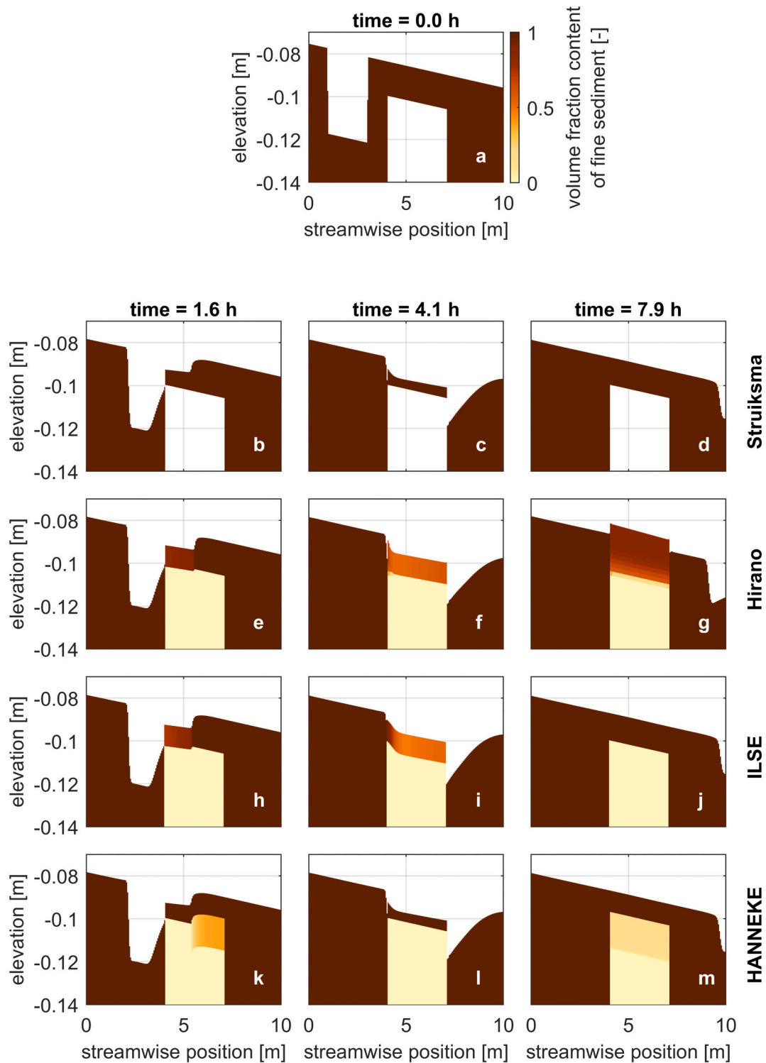
Fig. 8. Initial condition (a) and model results at different times (in columns) applying the model by Struiksmma (top row), the model by Hirano (second row from above), the ILSE flux (third row from above) and the HANNEKE model (fourth row from above) to a case in which coarse sediment is immobile.
