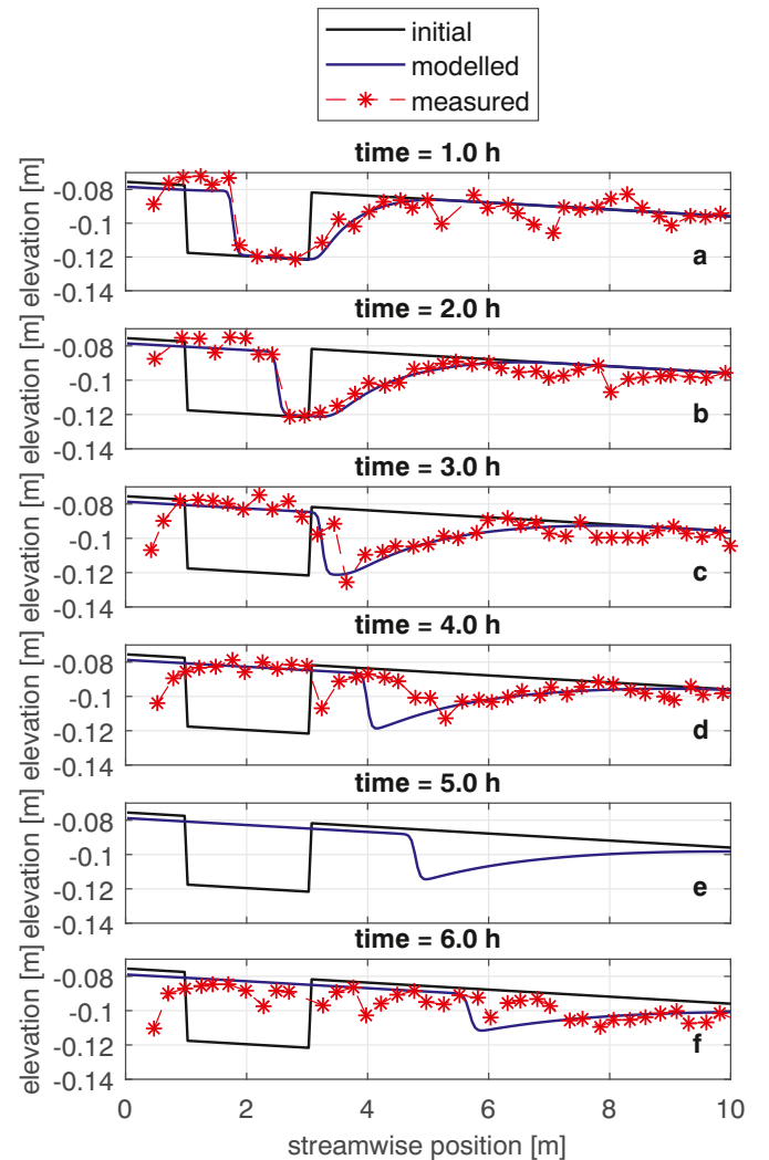
Fig. 7. Measured data and modelled results of the reference experiment (i.e., without a fixed layer) by Struiksma (1999). No measurements were available at 5 h.
