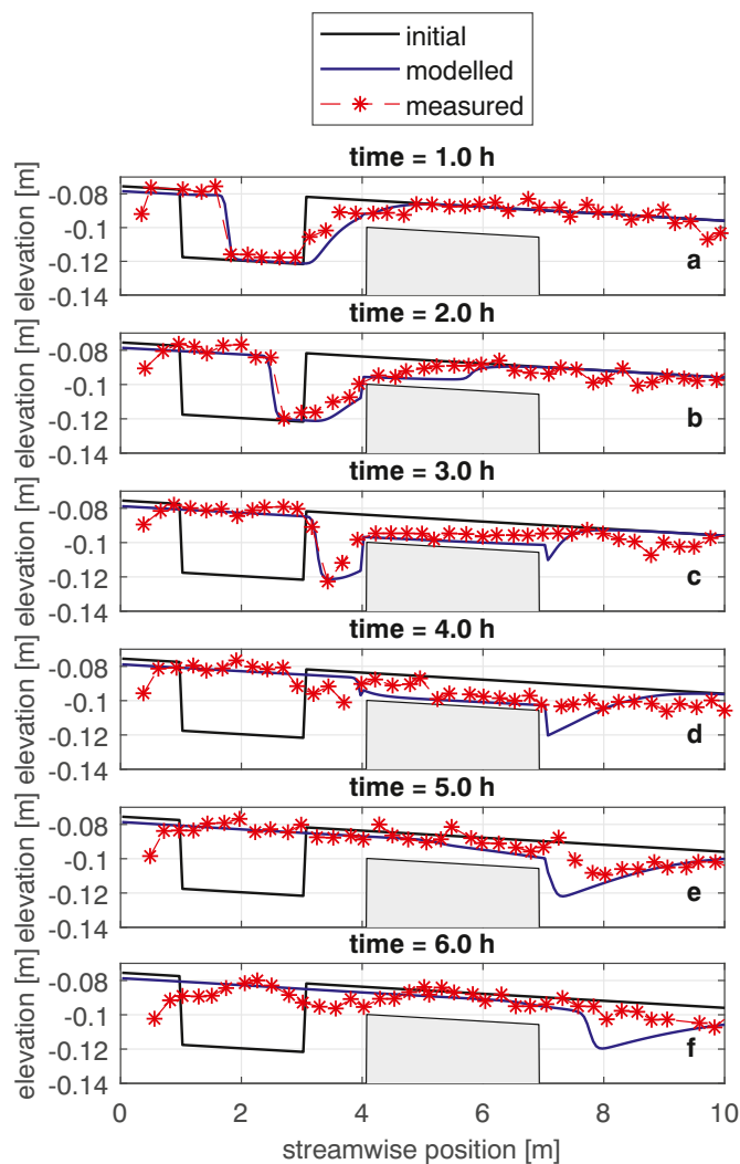
Fig. 9. Measured data of the experiment by Struiksmas (1999) with a fixed layer and model results using the Struiksmas model.
