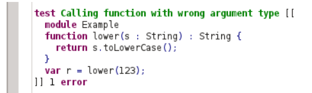
(c) A passing test case specifying negative test condition.
