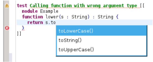
(a) Content completion for the language under test.
