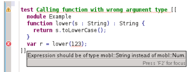
(b) Online evaluation of tests and error markers.
