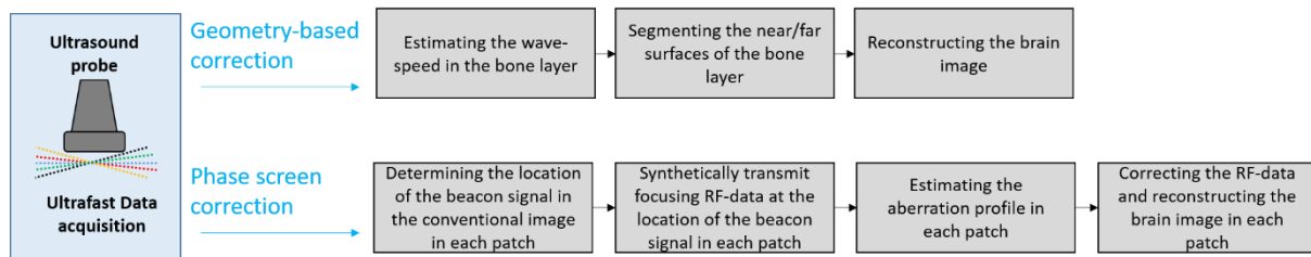
Figure 1. The block diagram showing the processing procedure for the geometry-based and phase-screen aberration correction techniques when an ultrafast imaging sequence (multi-angle plane wave) is used for data acquisition.
