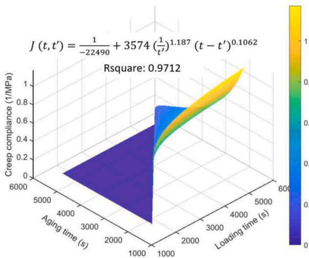
Fig. 12. Calibrated creep compliance surface.
