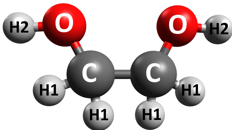
Figure A3: Structure and atom labels of ethylene glycol.
