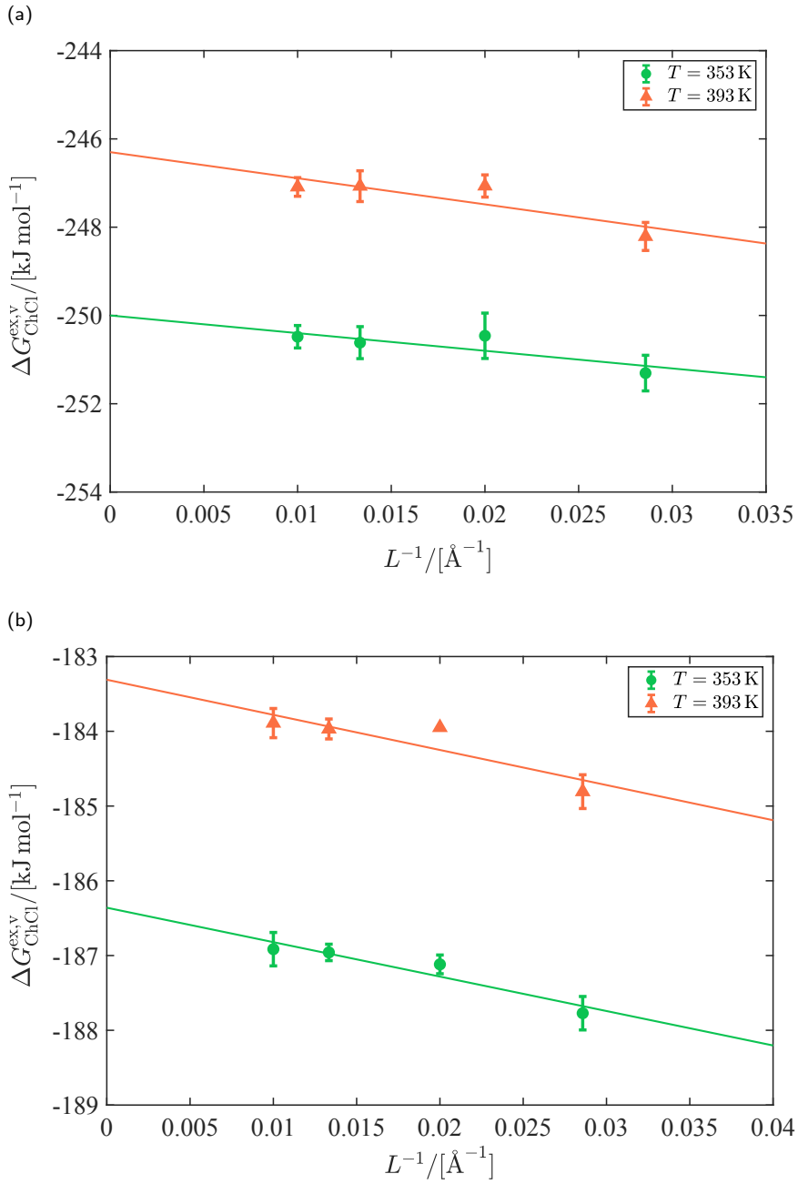
Figure 4.3: Computed vapor phase excess Gibbs energies of choline chloride in (a) ChClEg, and (b) ChClU, as a function of the inverse of the box size, at different temperatures. The solid lines depict the linear fits used for the extrapolation of \Delta G_{\text{ChCl}}^{\text{ex,v}} to infinite volume.
