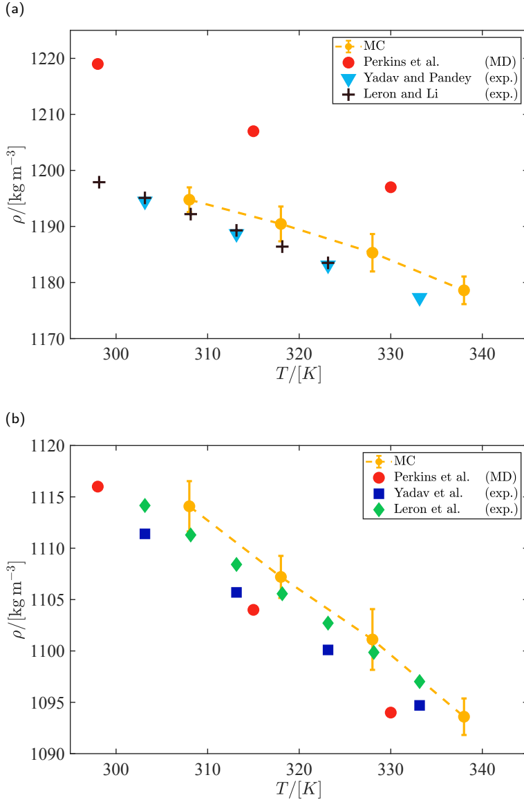
Figure 3.1: Computed densities of (a) ChCIU and (b) ChClEg, at various temperatures and 1 bar from MC simulations (orange circles and dashed line), compared to the MD results by Perkins et al. [61, 121] (red circles), and experimental data by Yadav and Pandey [181] (blue triangles), Leron and Li [235] (black pluses), Yadav et al. [36] (blue squares), and Leron et al. [265] (green diamonds). The small differences between the computed densities from MC and the MD simulation results of Perkins et al. [61, 121] may be due to the exclusion of improper torsion and bond-stretching energies from the MC simulations, and/or the differences in the use of tail corrections, shifting of the LJ potential, cutoff radius, and system size.
