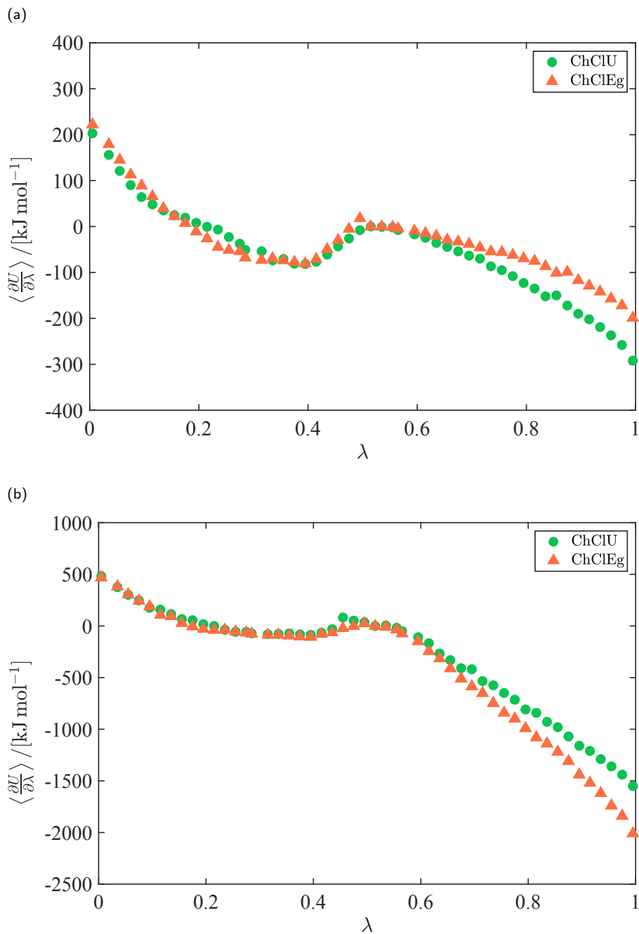
Figure 4.2: Ensemble averages of the derivative of the total energy with respect to \lambda , as a function of \lambda , for (a) the HBD (urea or ethylene glycol), and (b) choline chloride in ChClU (at 393 K) and ChClEg (at 353 K), from the liquid phase simulations.
