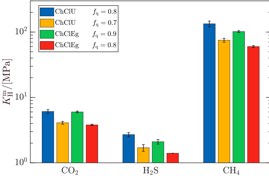
Figure 3.5: Comparison of the computed Henry coefficients (molality-based) of \text{CO}_2 , \text{H}_2\text{S} , and \text{CH}_4 in ChClU and ChClEg, using the GAFF force field parameters with different ionic charge scaling factors ( f_q ) for the DESs.
