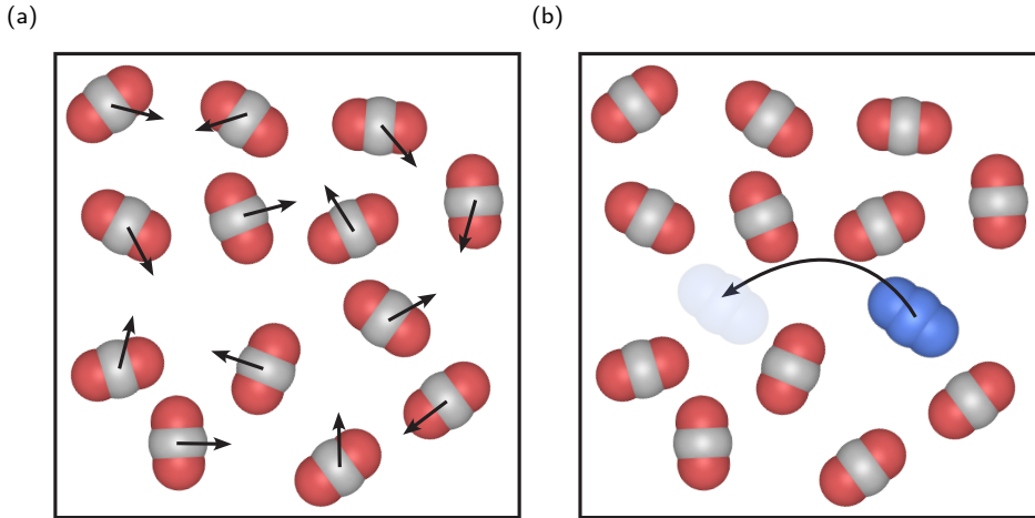
Figure 1.2: Schematic representations of (a) Molecular Dynamics (MD) and (b) Monte Carlo simulations for CO 2 . In MD simulations, atoms/molecules move collectively according to the resultant inter-atomic forces, based on Newton's equations of motion. In MC simulation, trial moves are performed (e.g., translation or reinsertion) for randomly selected molecules (shown in blue in (b)) or groups of molecules. These trial moves are accepted or rejected based on the detailed balance condition [69]. Collective trial moves can also be performed in MC simulations, e.g., see Refs. [80, 81].
