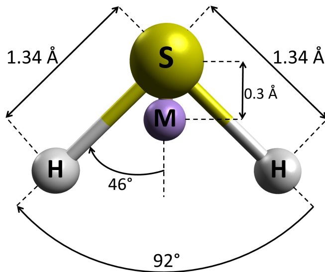
Figure A15: Structure and atom labels of hydrogen sulfide [261].
