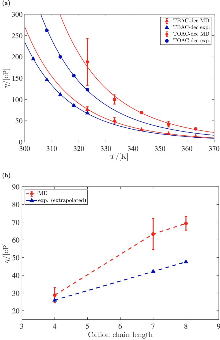
Figure 5.3: Viscosities of the TRAC-dec DESs (a) as a function of temperature (THAC-dec data are not shown for clarity), and (b) as a function of the cation alkyl chain length at 343 K, compared with the experimental data by van Osch et al. [20], extrapolated to 343 K. The experimental viscosity data point of THAC-dec in (b) was obtained by interpolating the experimental viscosities of TBAC-dec and TOAC-dec with respect to the cation chain length, and is therefore not equal to the value reported by van Osch et al. [20]. The solid lines in (a) denote the fits to the Arrhenius equation (Eq. 2.6). The dashed lines in (b) are added to guide the eye. For clarity, error bars that are smaller than the symbol size are not shown.
