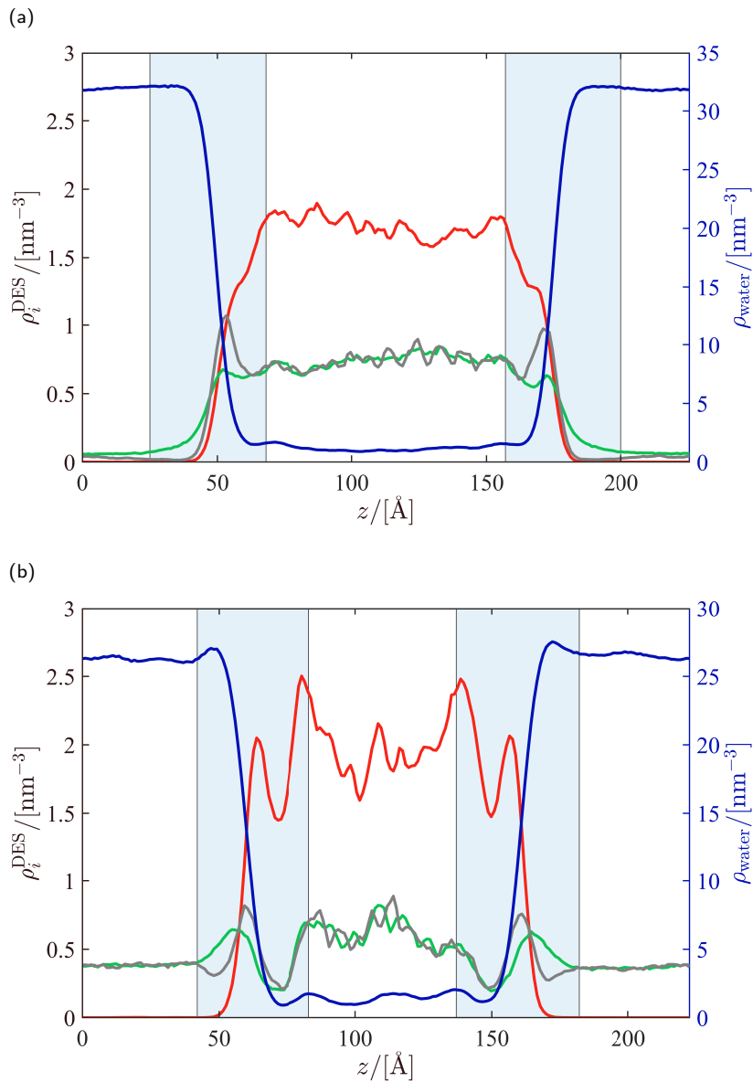
Figure A26: Computed number density profiles (number of molecules per \text{nm}^3 ) of DES components i (left vertical axis) and water (right vertical axis) in the TBAC-dec/water mixture at 343 K and 1 atm, using charge scaling factors of (a) f_q = 0.6 , and (b) f_q = 0.8 for the HBA (additional results from chapter 6). The red, green, gray, and blue colors correspond to decanoic acid (HBD), chloride (anion), choline (cation), and water, respectively. For the density profiles of decanoic acid and choline, the coordinates of the hydroxyl oxygen and the nitrogen atoms were used, respectively. The DES/water interfaces are indicated using blue shaded areas.
