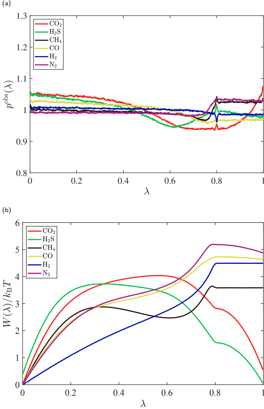
Figure 3.3: (a) Observed probability distributions of \lambda of the fractional molecules of various gases in ChCIU at 328 K and 1 bar (averaged over all independent runs). (b) The corresponding weight functions used to make the observed probability distributions of \lambda flat.
