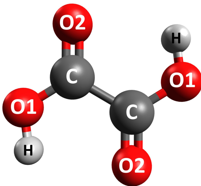
Figure A6: Structure and atom labels of oxalic acid.
