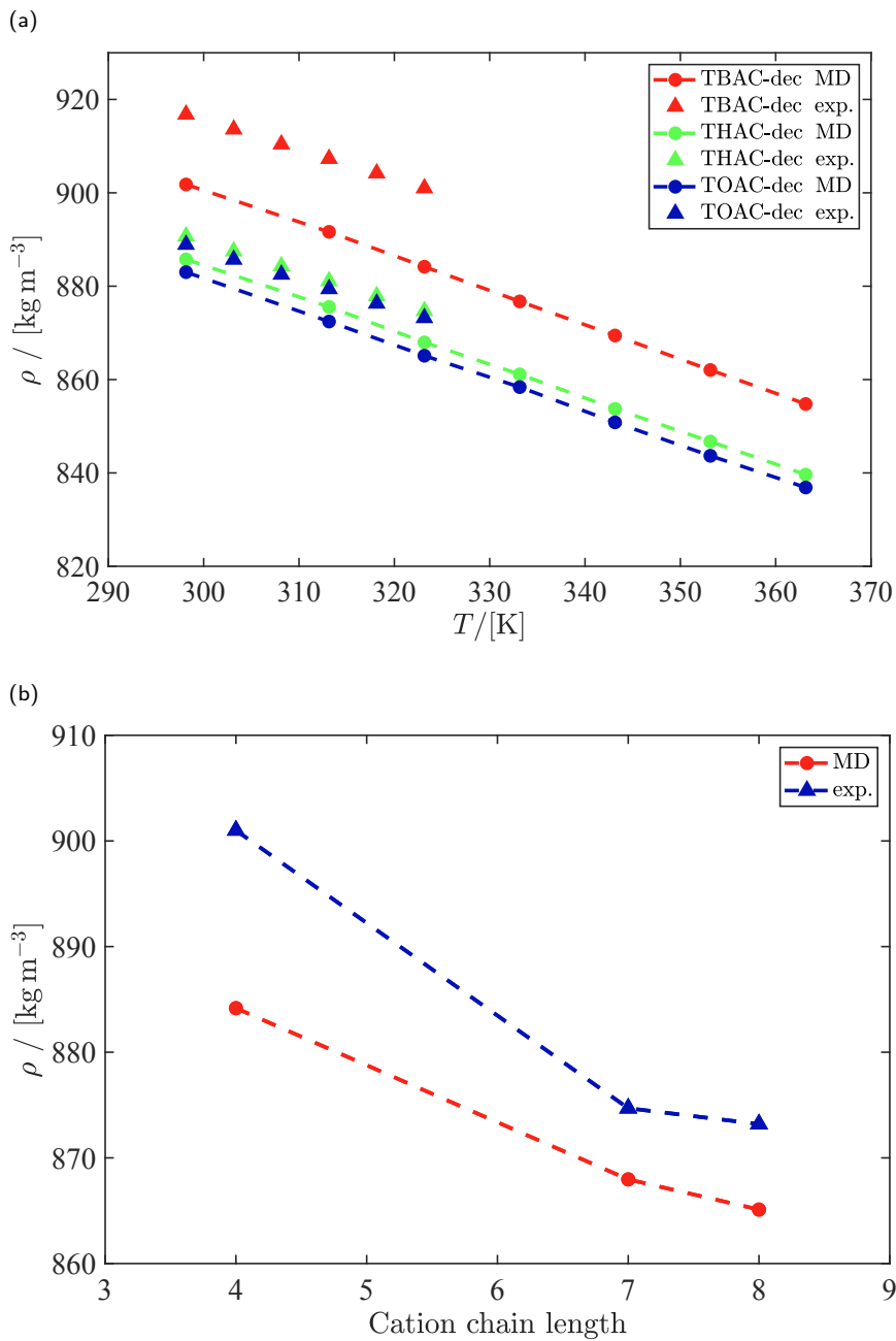
Figure 5.2: Densities of TBAC-dec, THAC-dec, and TOAC-dec (a) as a function of temperature, and (b) as a function of the cation alkyl chain length at 323 K, compared with the experimental data by van Osch et al. [20]. The dashed lines are added to guide the eye.
