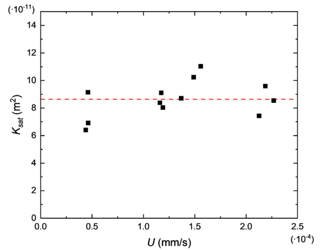
Fig. 3. Saturated permeability results.
