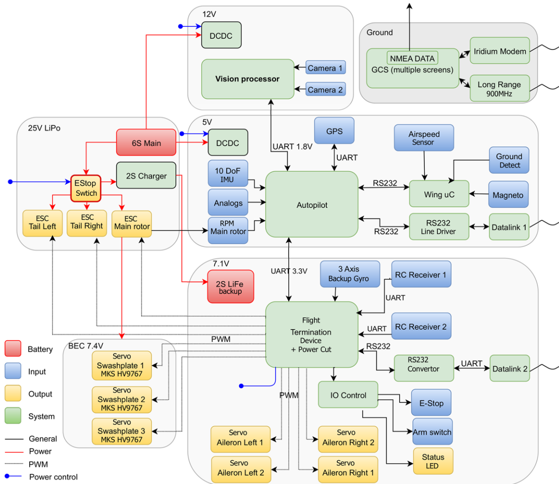
FIGURE 21 Schematic overview of the DelftaCopter electronics
