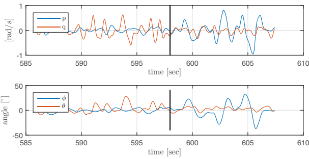
FIGURE 30 Manual test flight in attitude mode to confirm the observed coupling as seen in Figure 24 has been resolved. In this flight, a K_c of 0.5 was selected to yield the best results. Before time t = 598 the test pilot was applying mainly pitch commands, and after mainly roll commands while keeping the vehicle in the flight area
