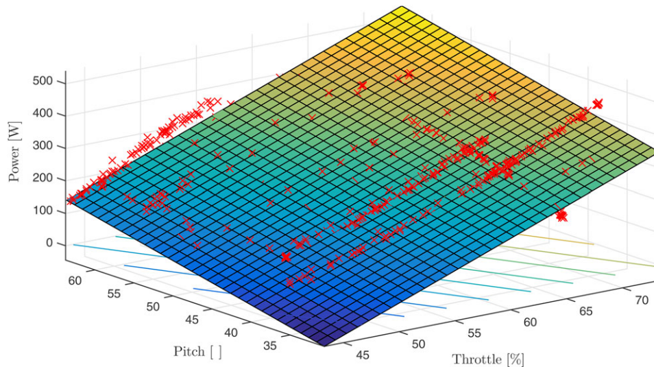
FIGURE 20 Measured power in function of pitch and throttle and planar fit showing rpm and pitch can be exchanged while keeping the same used power
