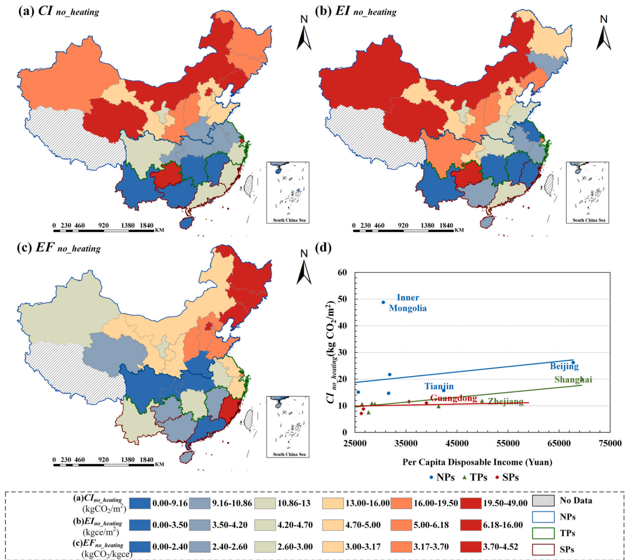
Fig. 5. The provincial URB condition of CI_{no\_heating} in 2019. (Note: Fig. 5a, b, and c represent the spatial distribution in CI_{no\_heating} , EI_{no\_heating} , and EF_{no\_heating} , respectively. CI , EF , and EI represent carbon emission unit area, emission factor and energy consumption unit area, respectively. NPs, TPs and SPs represents north, transitional and south provinces, respectively.)
