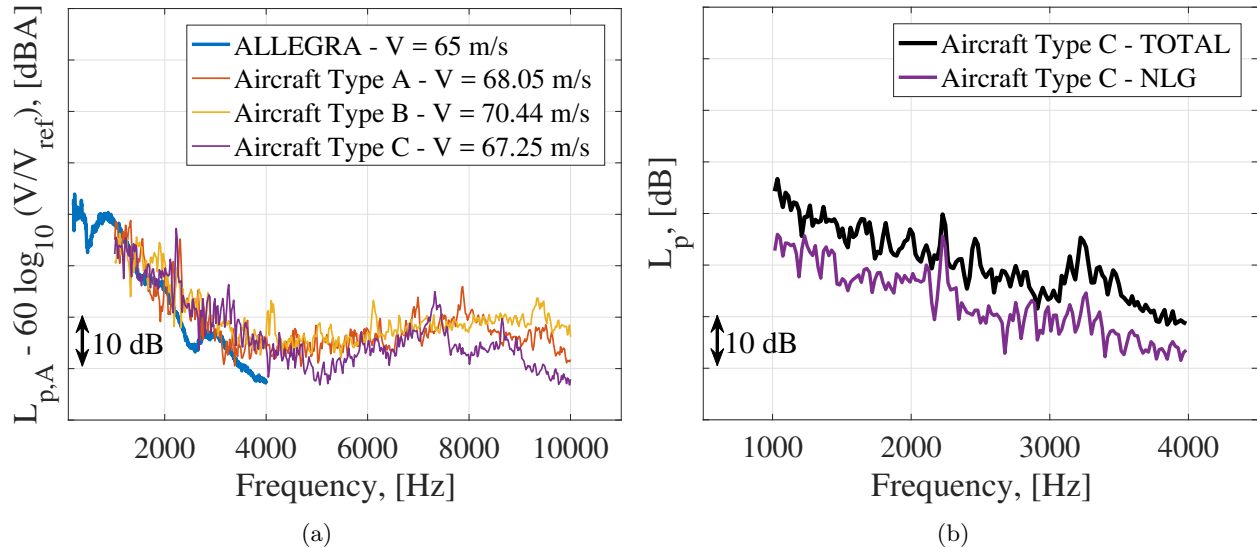
Figure 17: (a) Integrated A-weighted narrow-band frequency spectra of the NLG for an example flyover of each aircraft type. The spectrum of the ALLEGRA model with V_{ref} = 65 m/s is also plotted for comparison. (b) Zoomed-in spectra comparison for an Aircraft Type C flyover between the NLG and the total aircraft ( V = 67.25 m/s)
