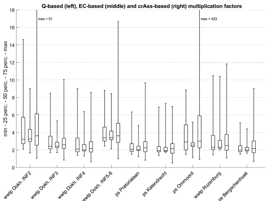
Fig. 3. Boxplot with Q-based (left), EC-based (middle) and crAssphage-based (right) multiplication factors per catchment area. Each boxplot gives the minimum, 25th percentile, the median, the 75th percentile and the maximum value by the whiskers.
