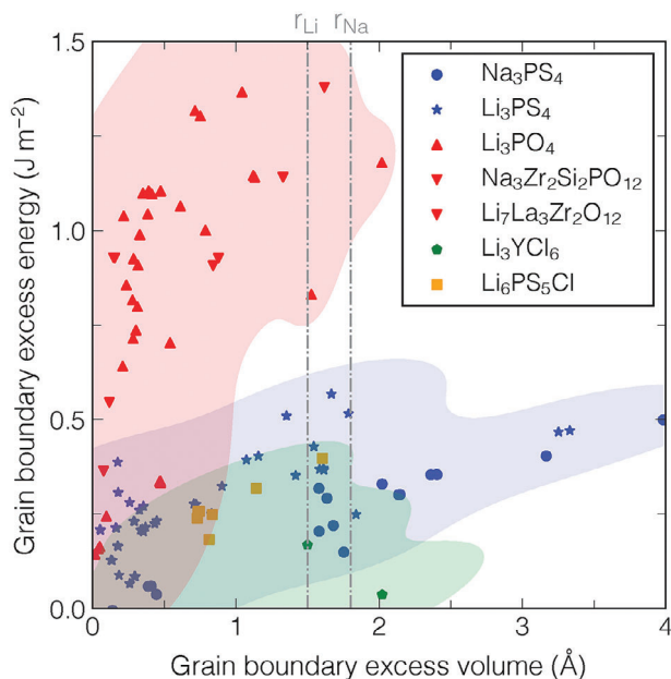
Figure 2. Relationship between the excess volume \Omega (in Å) and excess energy \sigma (in J m -2 ) of GB models of different SEs. Each data point corresponds to a GB model. Gray lines mark the atomic radii of Li and Na. Colors categorize GBs that share “similar” chemistries.
